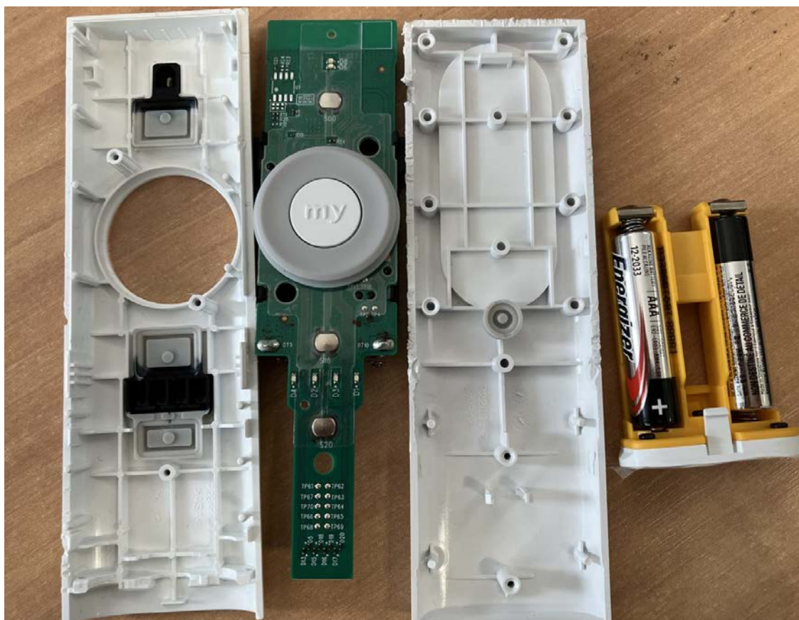
EUT- Inside View
