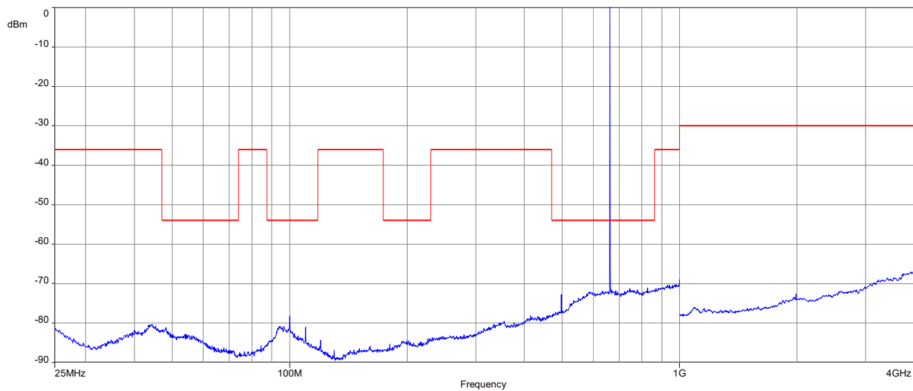
Plot 8: 662.875 MHz, spurious emissions, 25 MHz – 4 GHz
