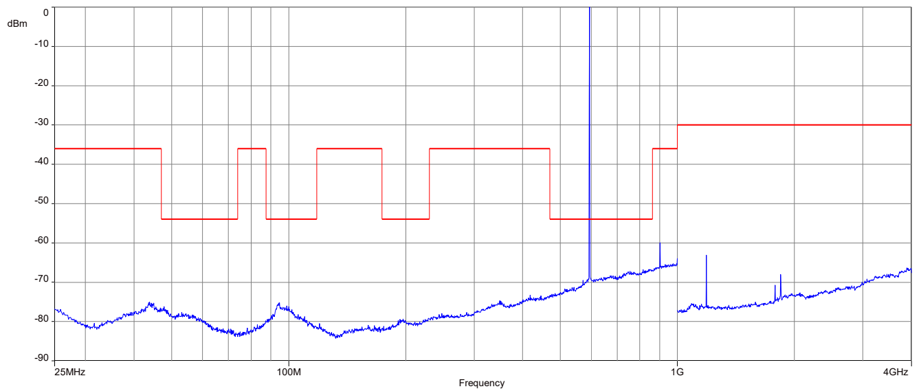
Plot 5: 594.000 MHz, spurious emissions, 25 MHz – 4 GHz
