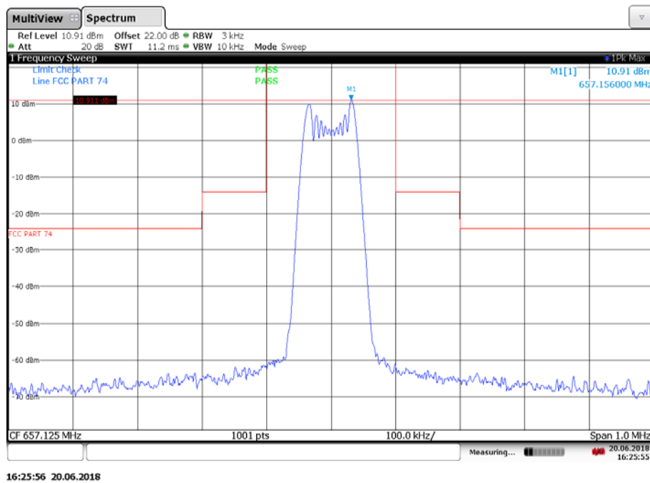
Plot 7: 657.125 MHz, spectrum mask
