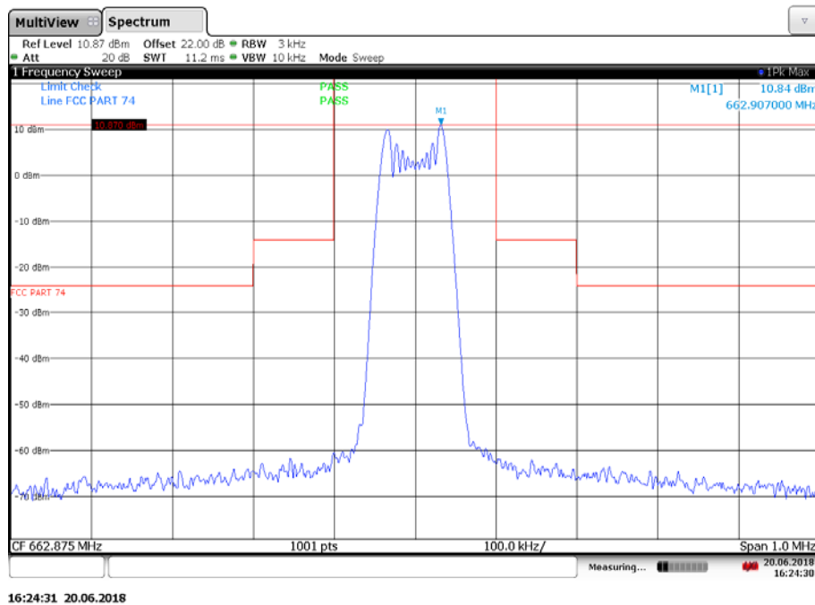
Plot 8: 662.875 MHz, spectrum mask
