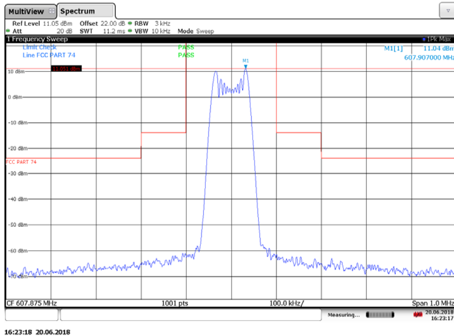
Plot 6: 607.875 MHz, spectrum mask
