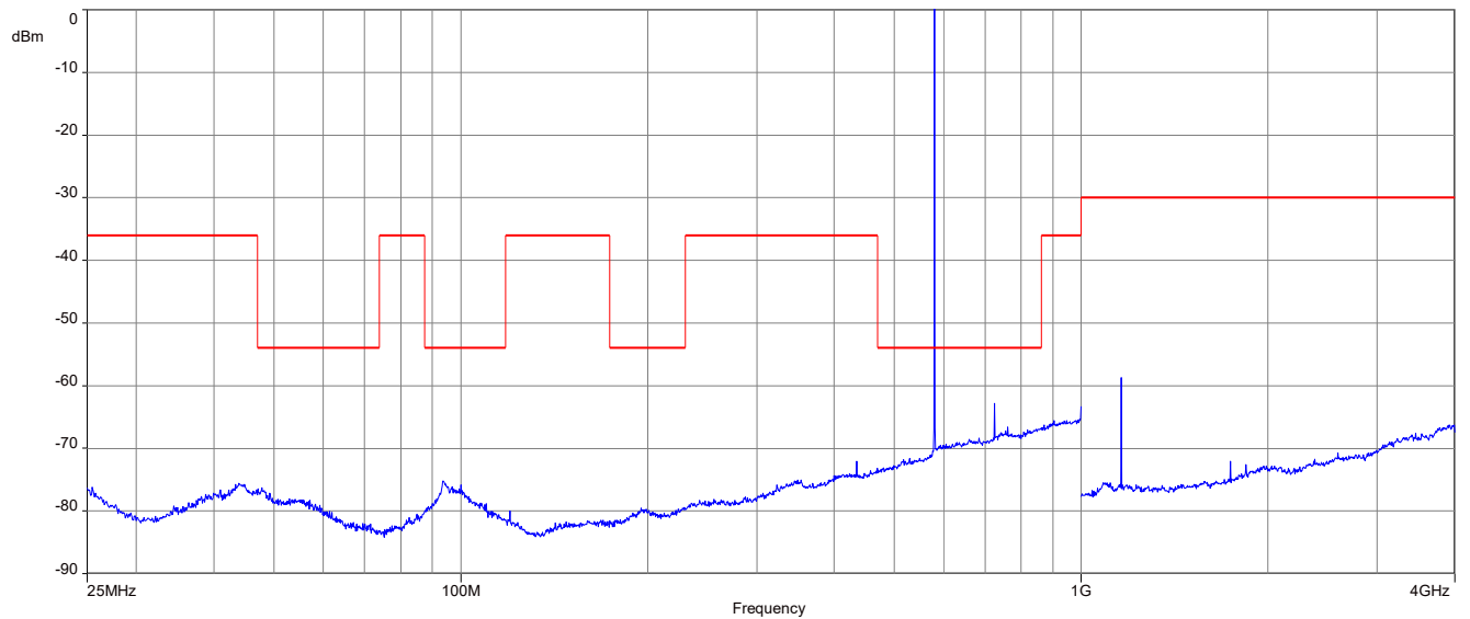
Plot 4: 580.000 MHz, spurious emissions, 25 MHz – 4 GHz
