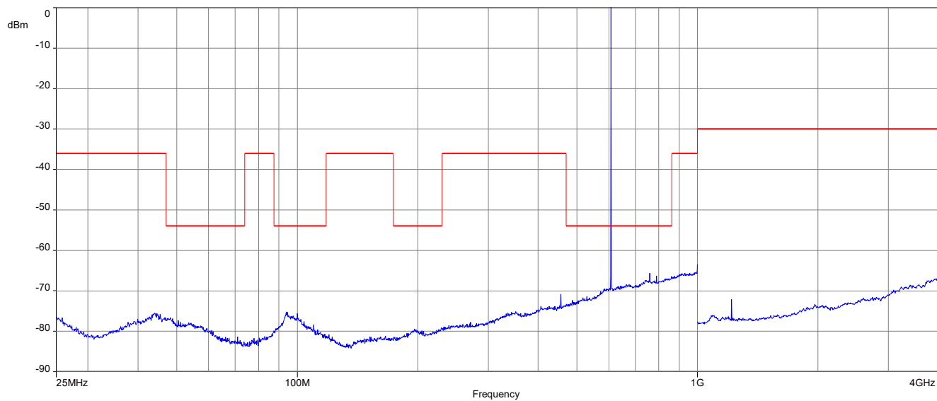
Plot 6: 607.875 MHz, spurious emissions, 25 MHz – 4 GHz
