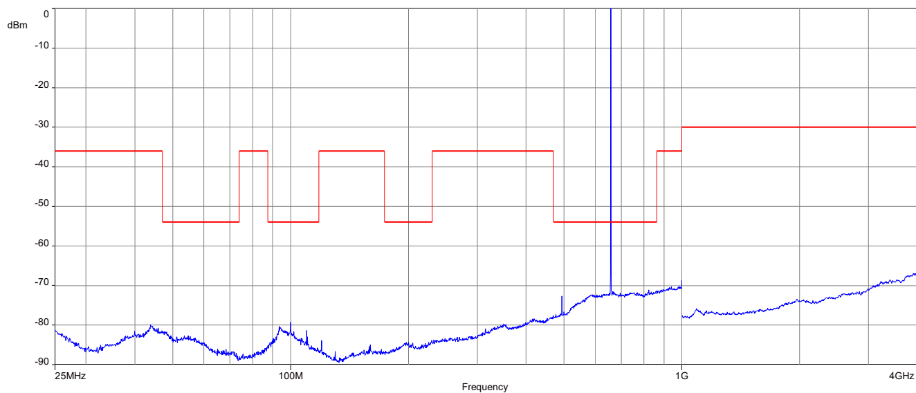
Plot 7: 657.125 MHz, spurious emissions, 25 MHz – 4 GHz
