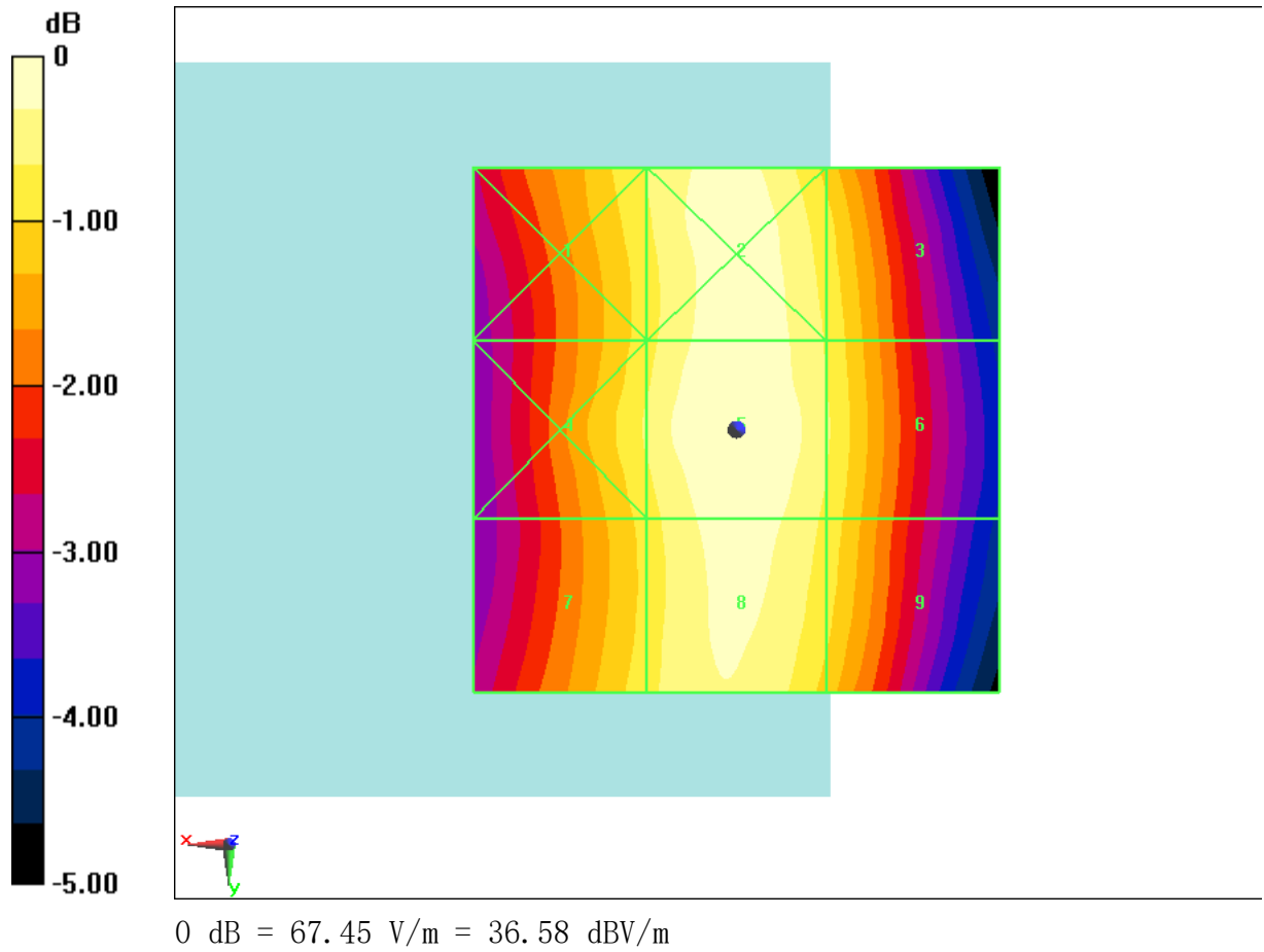
Fig B.1 HAC RF E-Field GSM 850 High
