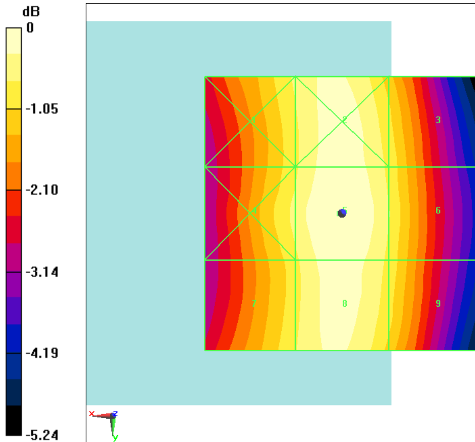
Fig B.3 HAC RF E-Field GSM 850 Low
