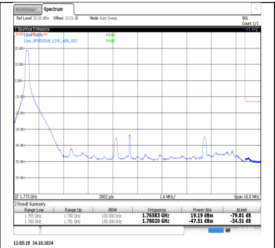
Band66-15MHz-16QAM-132597-1RB#74-PASS
