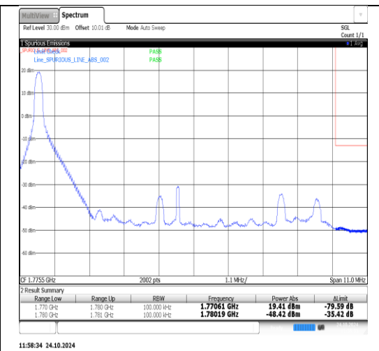
Band66-10MHz-16QAM-132622-1RB#49-PASS
