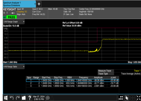
N2(40M)_DFT-s- OFDM_QPSK_Outer_Full_Low_CH
