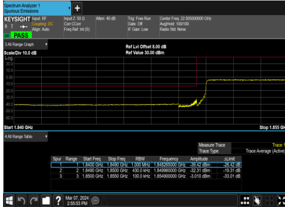
N2(40M)_DFT-s- OFDM_BPSK_Outer_Full_Low_CH
