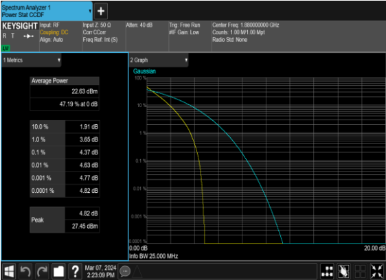
N2(20M)_DFT-s-OFDM_PI_2- BPSK_Outer_Full_Mid_CH
