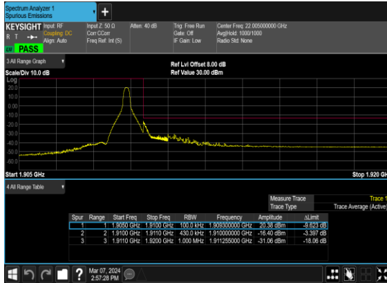
N2(40M)_DFT-s- OFDM_BPSK_Edge_1RB_Right_High_CH
