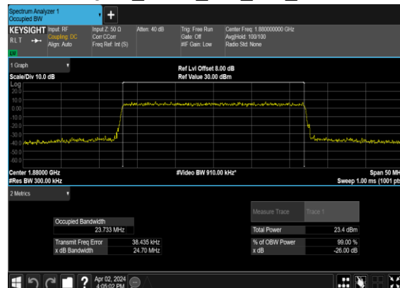
N2(25M)_CP-OFDM_256 QAM_Outer_Full_Mid_CH
