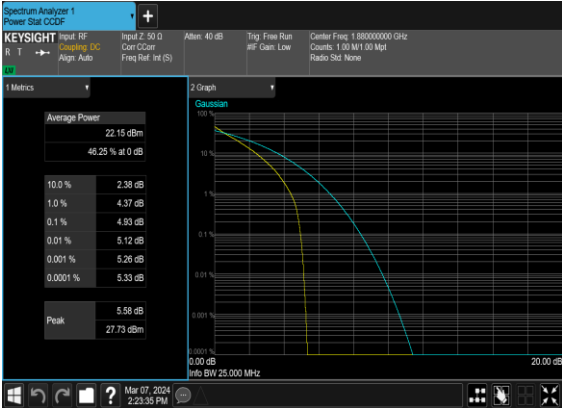
N2(20M)_DFT-s- OFDM_QPSK_Outer_Full_Mid_CH
