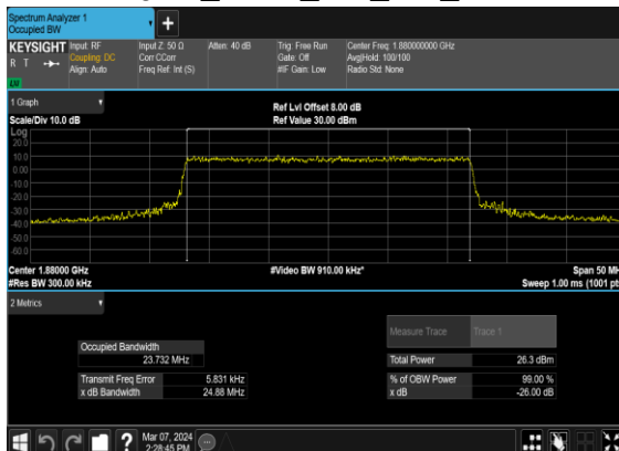
N2(25M)_CP-OFDM_64 QAM_Outer_Full_Mid_CH
