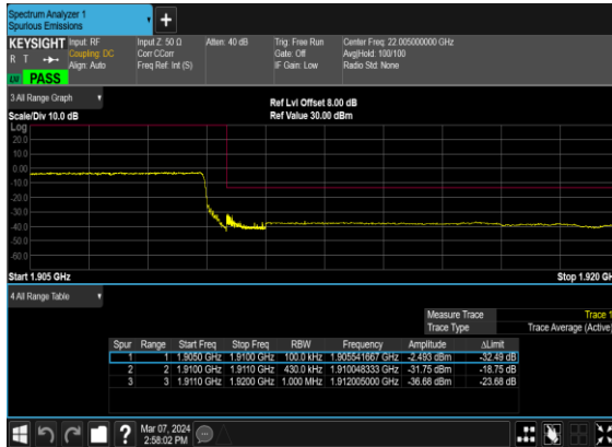
N2(40M)_DFT-s- OFDM_BPSK_Outer_Full_High_CH
