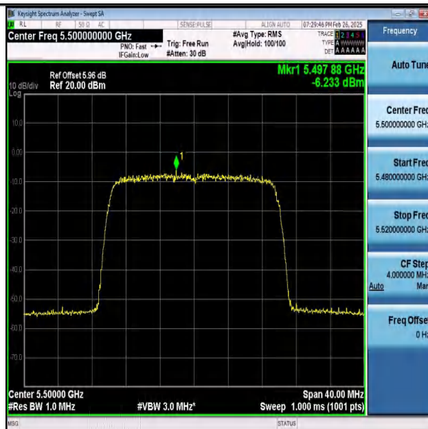
802.11ax (HE20)-Ant1-5500-PASS
