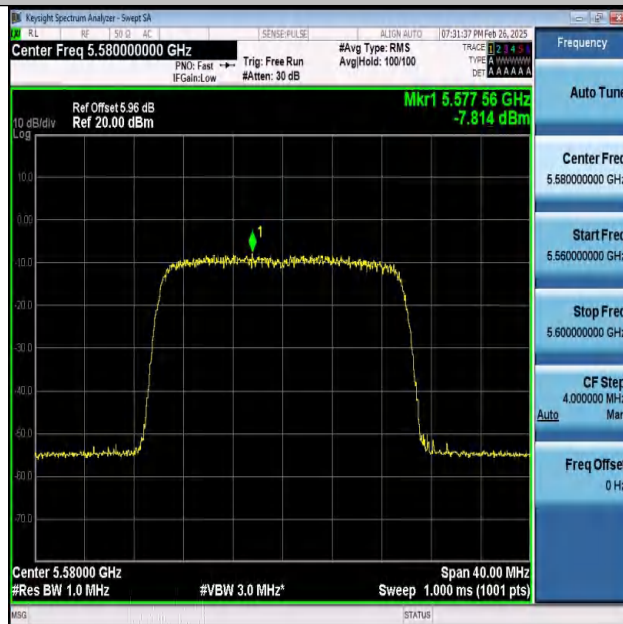
802.11ax (HE20)-Ant1-5580-PASS
