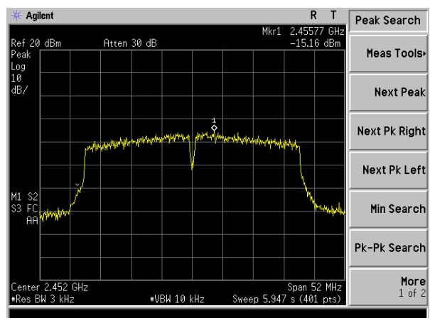
(802.11n40) channel 9
