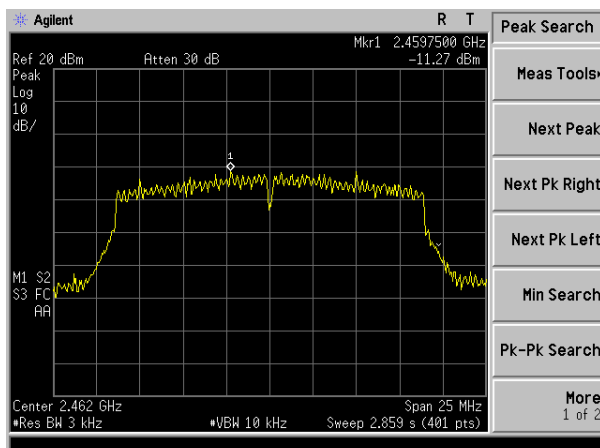
(802.11n20) channel 11
