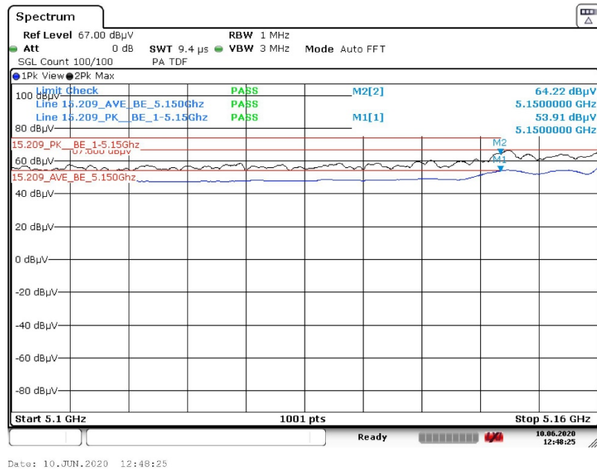
Plot 1: Transmitting on 5180 MHz a mode 20 MHz ch
