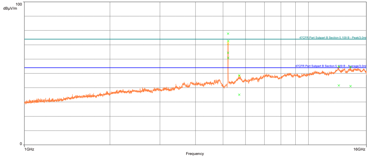
Plot 8 Transmitting on 5210 MHz ac mode 20 MHz ch
