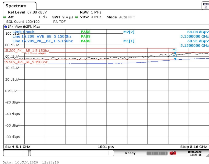
Plot 5 Transmitting on 5190 MHz ac mode 40 MHz ch
