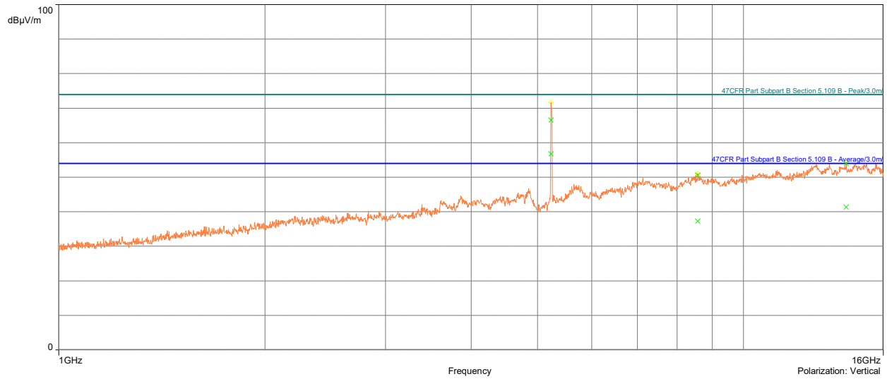
Plot 9 Transmitting on 5240 MHz ac mode 20 MHz ch
