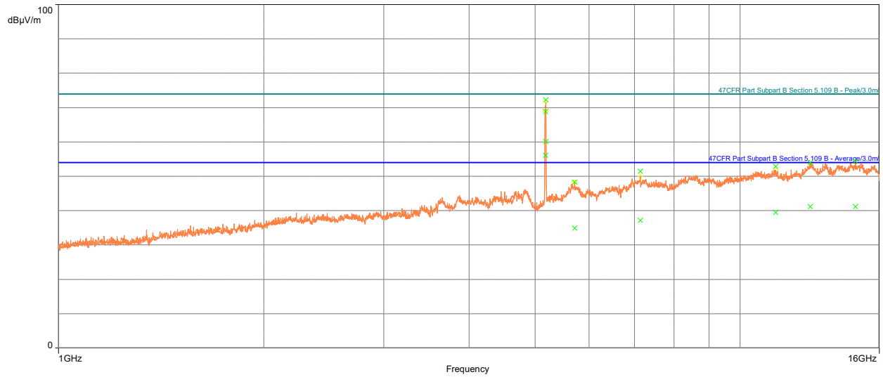
Plot 7 Transmitting on 5180 MHz ac mode 20 MHz ch
