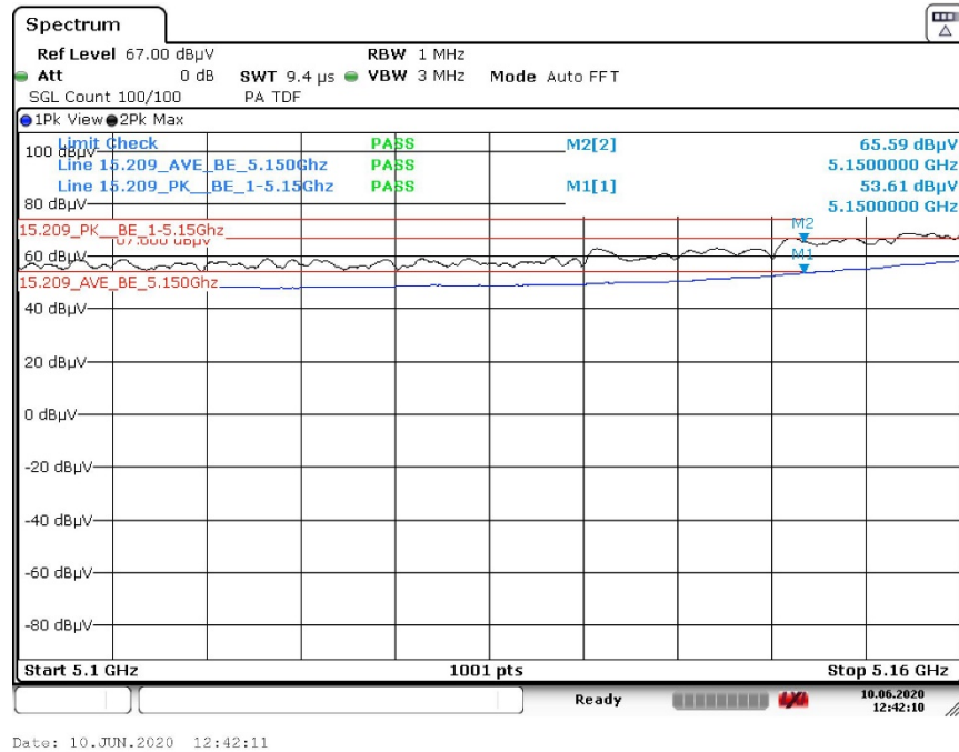
Plot 4 Transmitting on 5200 MHz ac mode 20 MHz ch
