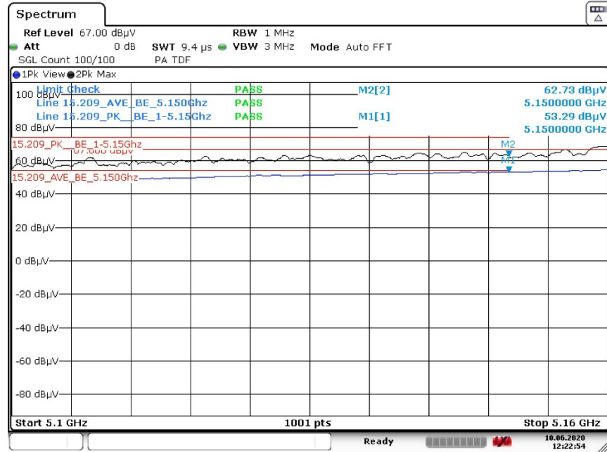
Plot 6 Transmitting on 5210 MHz ac mode 80 MHz ch
