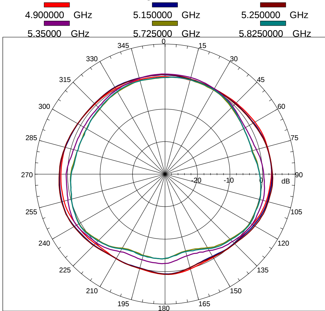
Far-field amplitude of V H-PLANE.nsi
