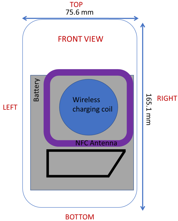
Figure E-2 NFC Antenna Locations
