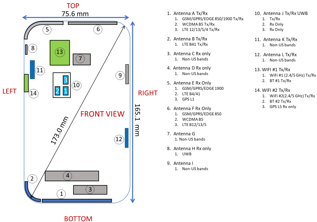
Figure E-1 DUT Antenna Locations
