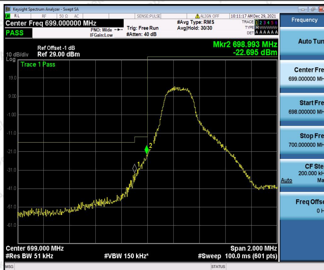
Band12-3MHz-16QAM-23025-1RB#14
