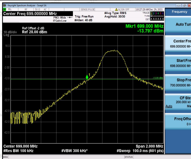
Band12-5MHz-16QAM-23035-1RB#24
