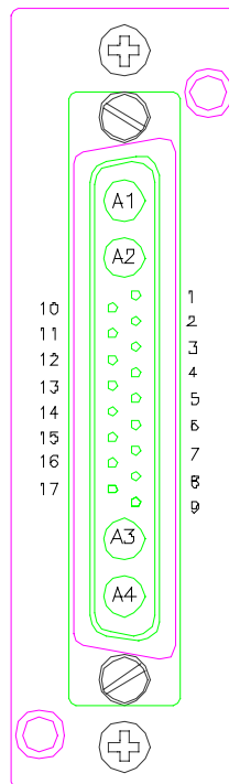
Figure 2-1. Power, Alarm, Control, and RF Connector (D-SubMiniature 21WA4, Male Connector)
