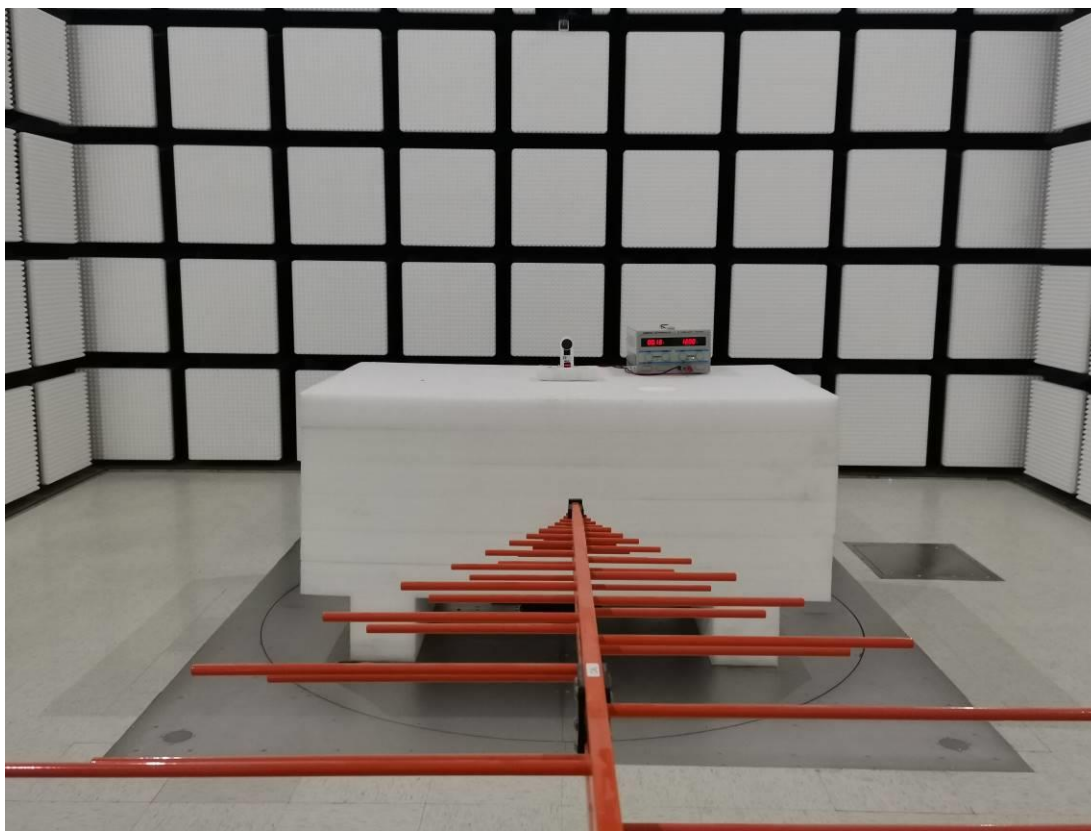
Radiated Emission Below 1GHz View DC 24V
