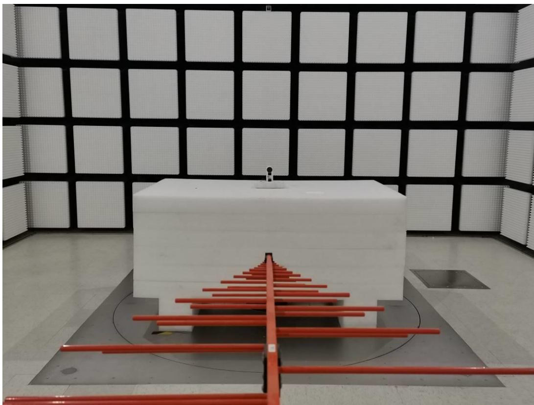
Radiated Emission Below 1GHz View AC
