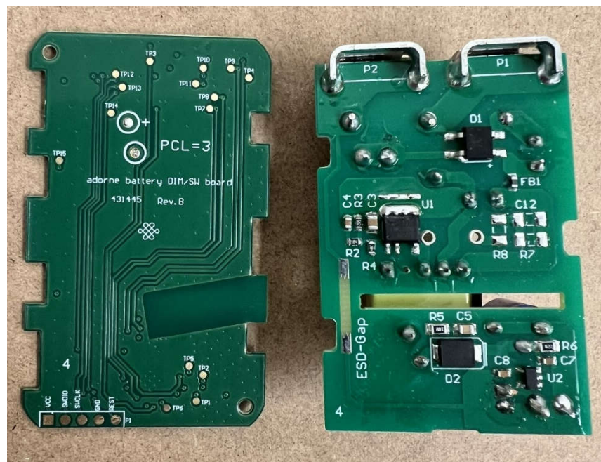
WNAL24 RF Board Back Side (Left) – AC Board Top Side (Right)
