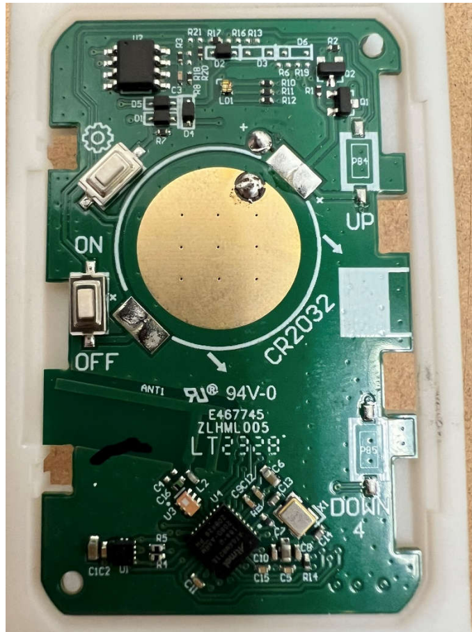
WNAL24 RF Board -Top
