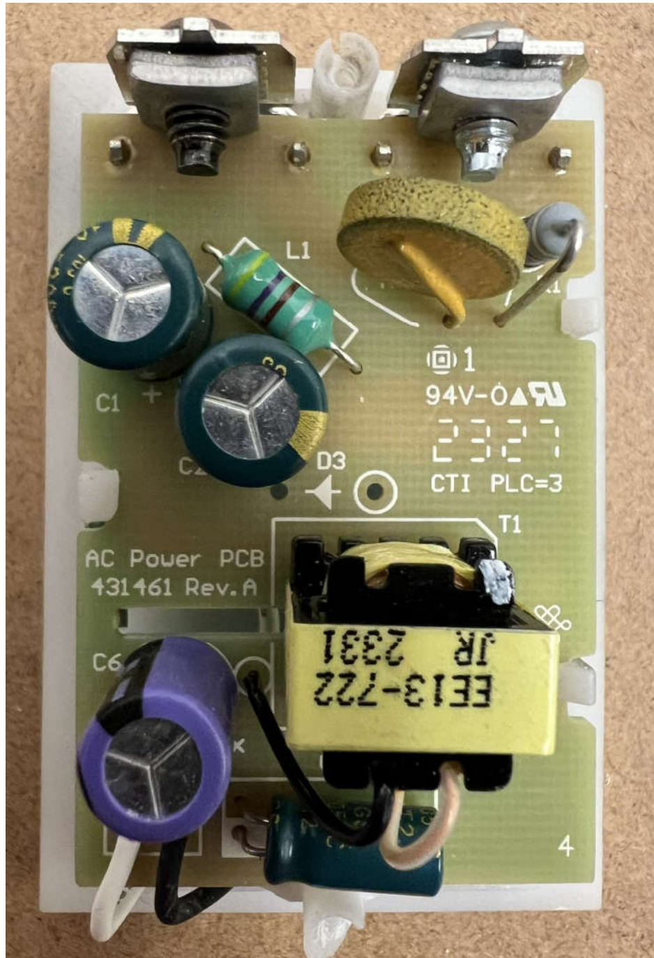
WNAL24 AC Board Back Side
