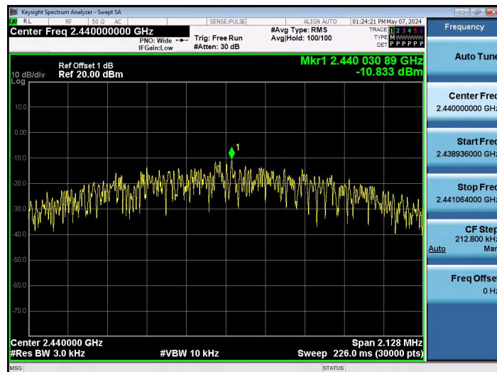
BLE_2M-Ant1-2440-PASS
