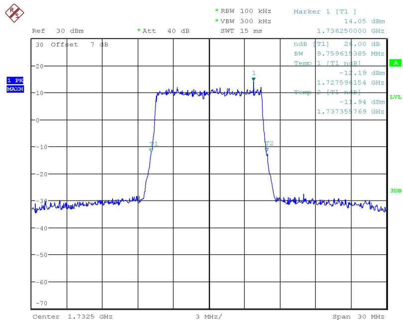
LTE band 4, 10MHz Bandwidth, 16QAM (-26dBc BW)
