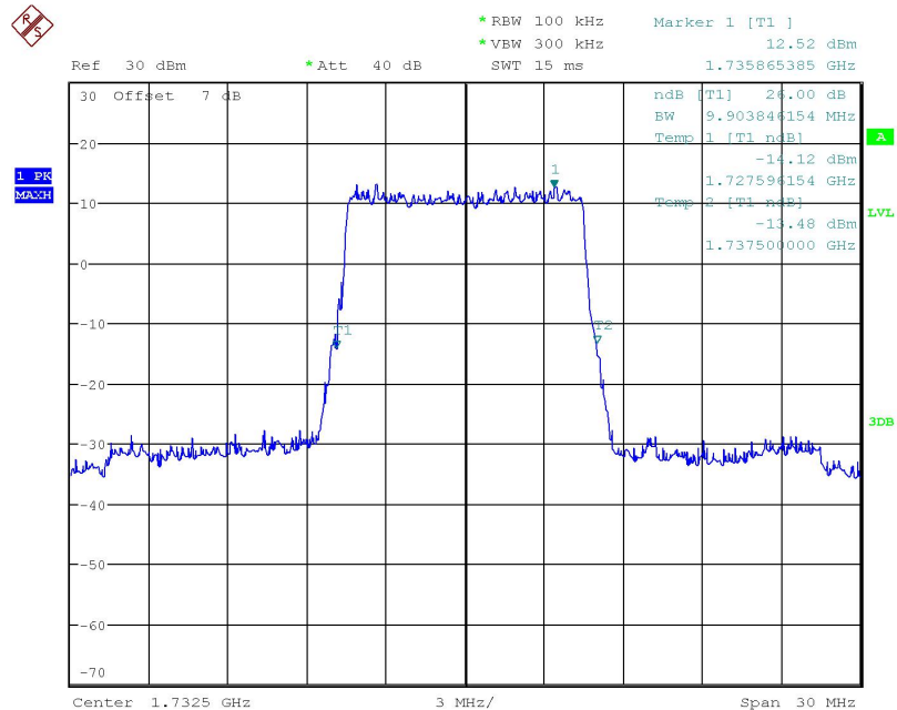
LTE band 4, 10MHz Bandwidth, QPSK (-26dBc BW)
