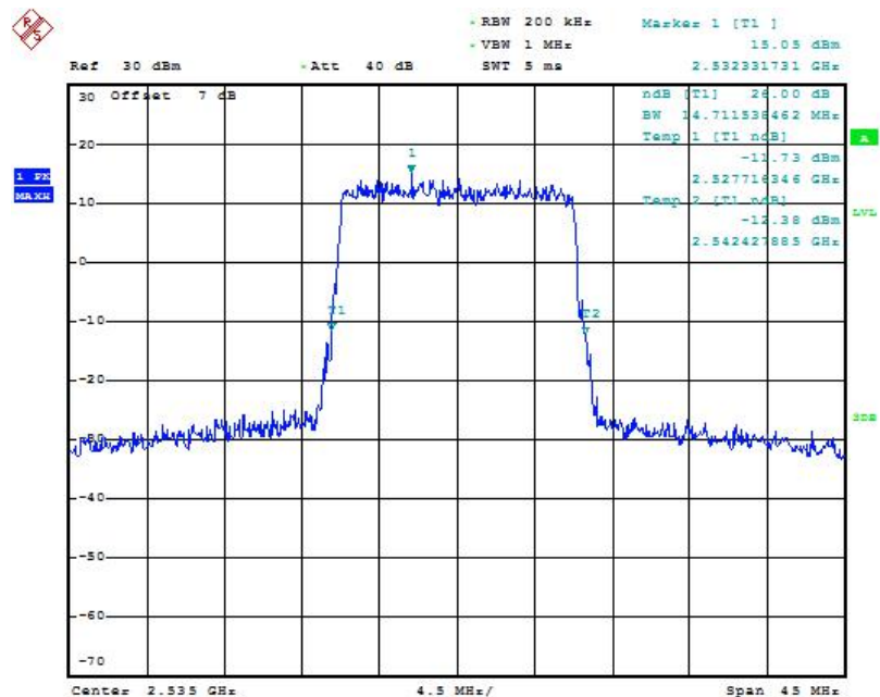
LTE band 7, 15MHz Bandwidth, 16QAM (-26dBc BW)
