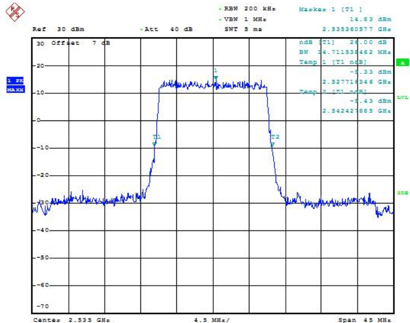
LTE band 7, 15MHz Bandwidth, QPSK (-26dBc BW)
