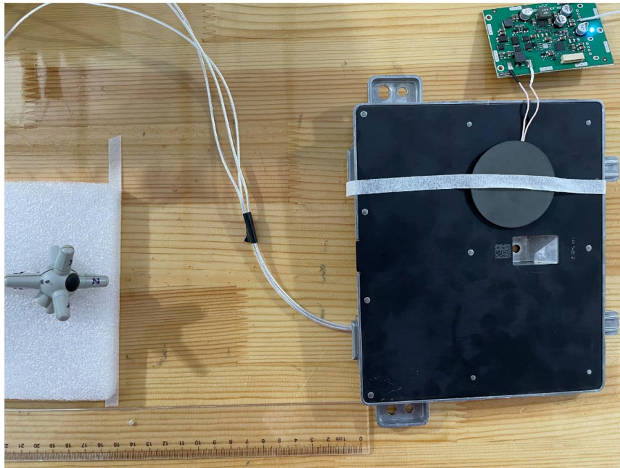
E-field Test Setup Photo of Position B(15cm)
