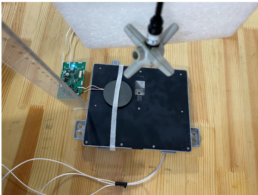
E-field Test Setup Photo of Position E(20cm)
