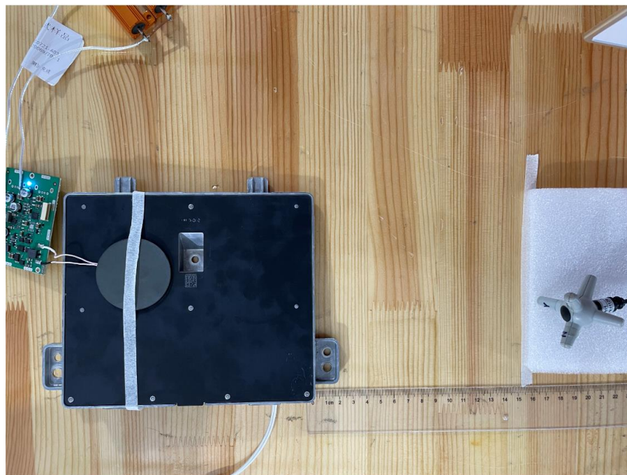
E-field Test Setup Photo of Position C(15cm)
