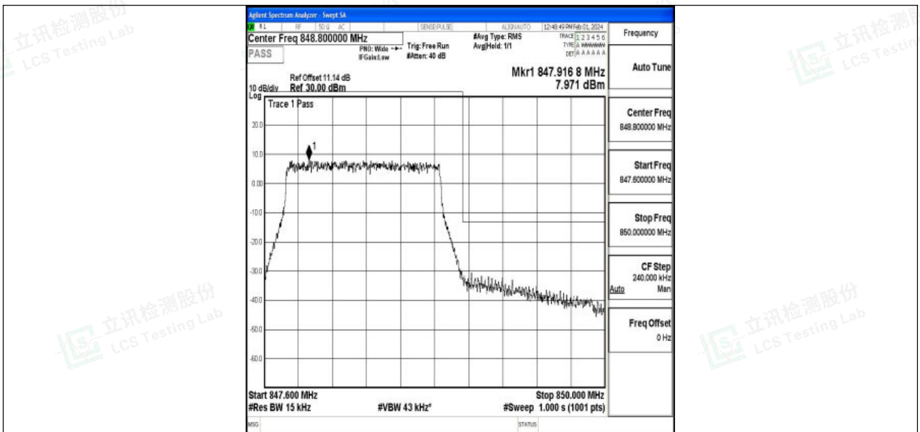
Band5_1.4MHz_16QAM_20643_6RB#0
