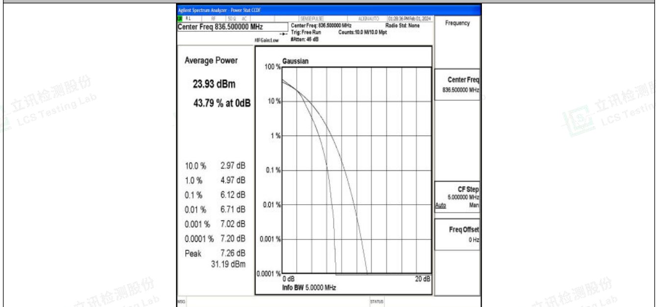
Band5-3MHz-16QAM-20525-15RB#0-PASS
