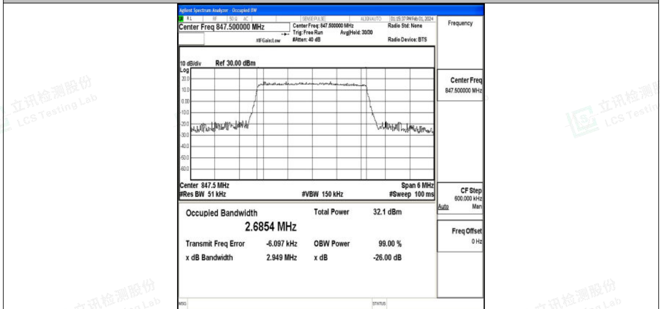
Band5-3MHz-16QAM-20635-15RB#0-PASS
