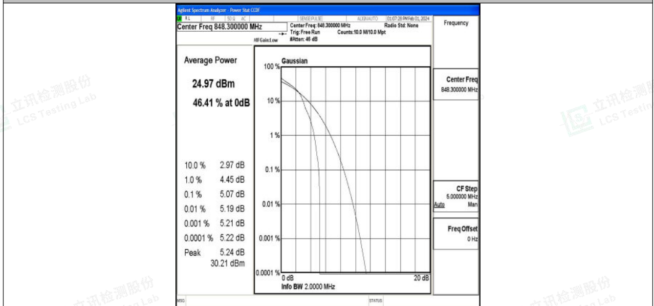
Band5-1.4MHz-16QAM-20643-1RB#0-PASS
