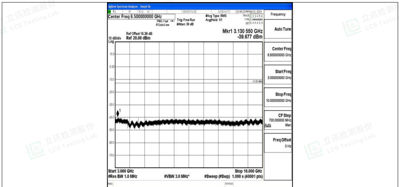
Band5_1.4MHz_QPSK_20407_1RB#0_3000~10000_3000~10000
