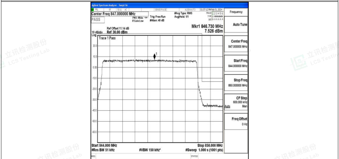
Band5_5MHz_QPSK_20625_25RB#0
