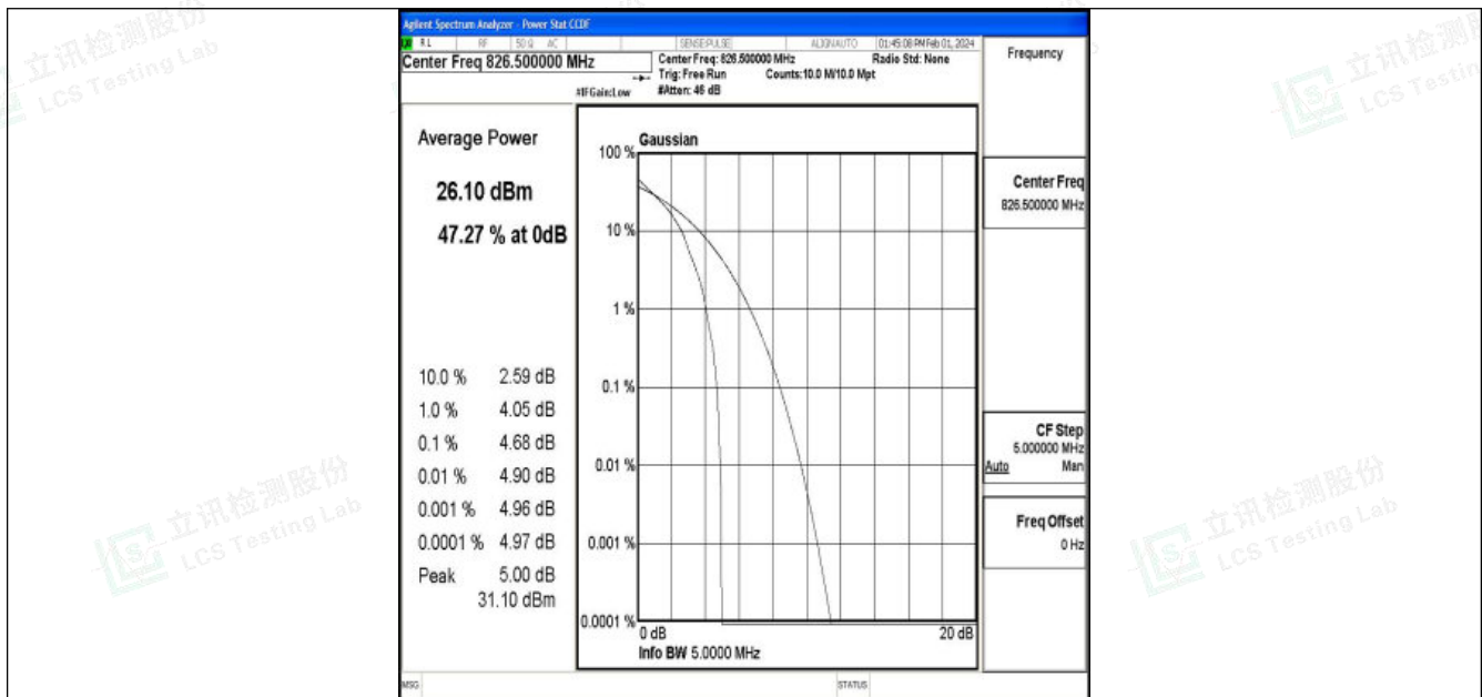
Band5-5MHz-QPSK-20425-1RB#0-PASS
