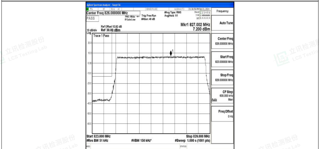
Band5_5MHz_QPSK_20425_25RB#0
