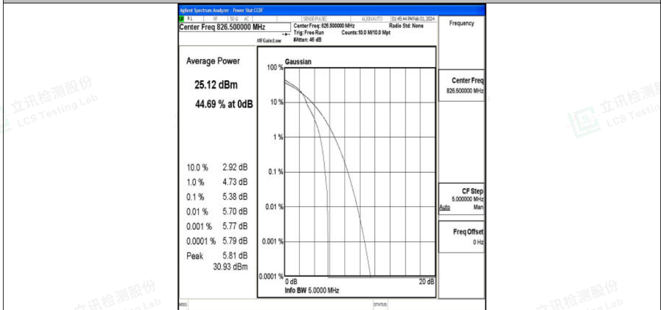
Band5-5MHz-16QAM-20425-1RB#0-PASS
