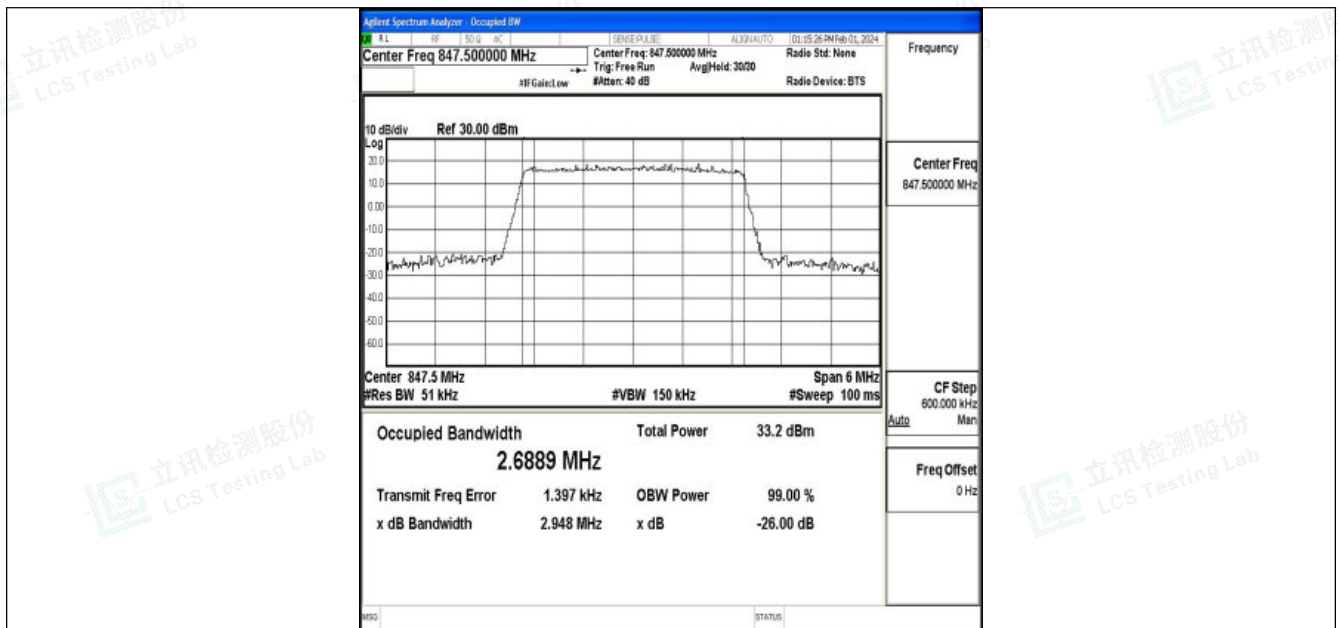
Band5-3MHz-QPSK-20635-15RB#0-PASS
