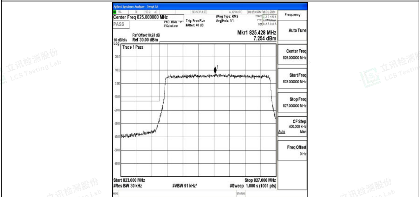
Band5_3MHz_QPSK_20415_15RB#0
