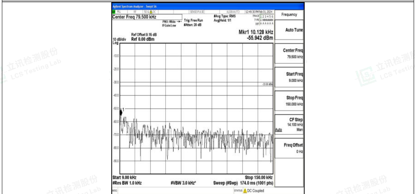
Band5_1.4MHz_16QAM_20407_1RB#0_0.009~0.15_0.009~0.15
