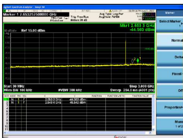
\pi/4 -DQPSK LOW CHANNEL, SPURIOUS 30 MHz ~ 3 GHz
