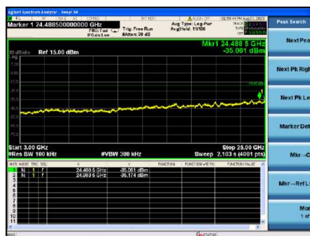
\pi/4 -DQPSK LOW CHANNEL, SPURIOUS 3 GHz ~ 25 GHz
