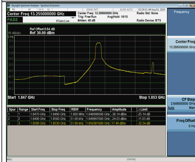
Band25_5MHz_QPSK_26065_1RB#0
