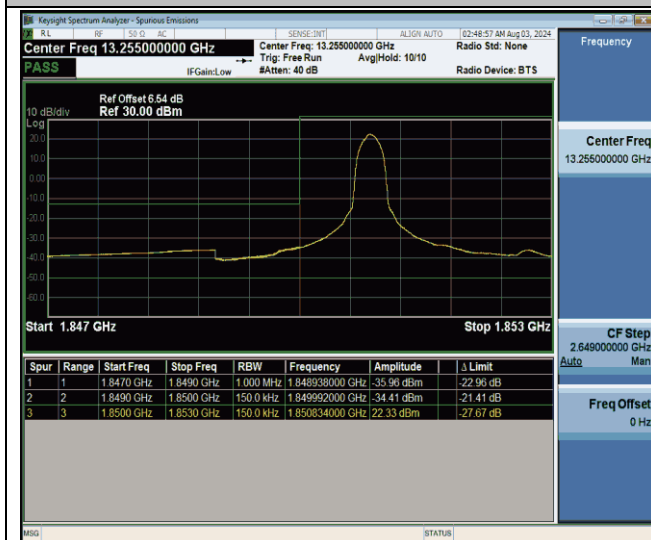
Band25_15MHz_QPSK_26115_1RB#0
