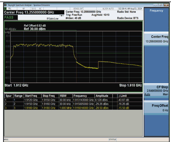
Band25_3MHz_QPSK_26675_15RB#0
