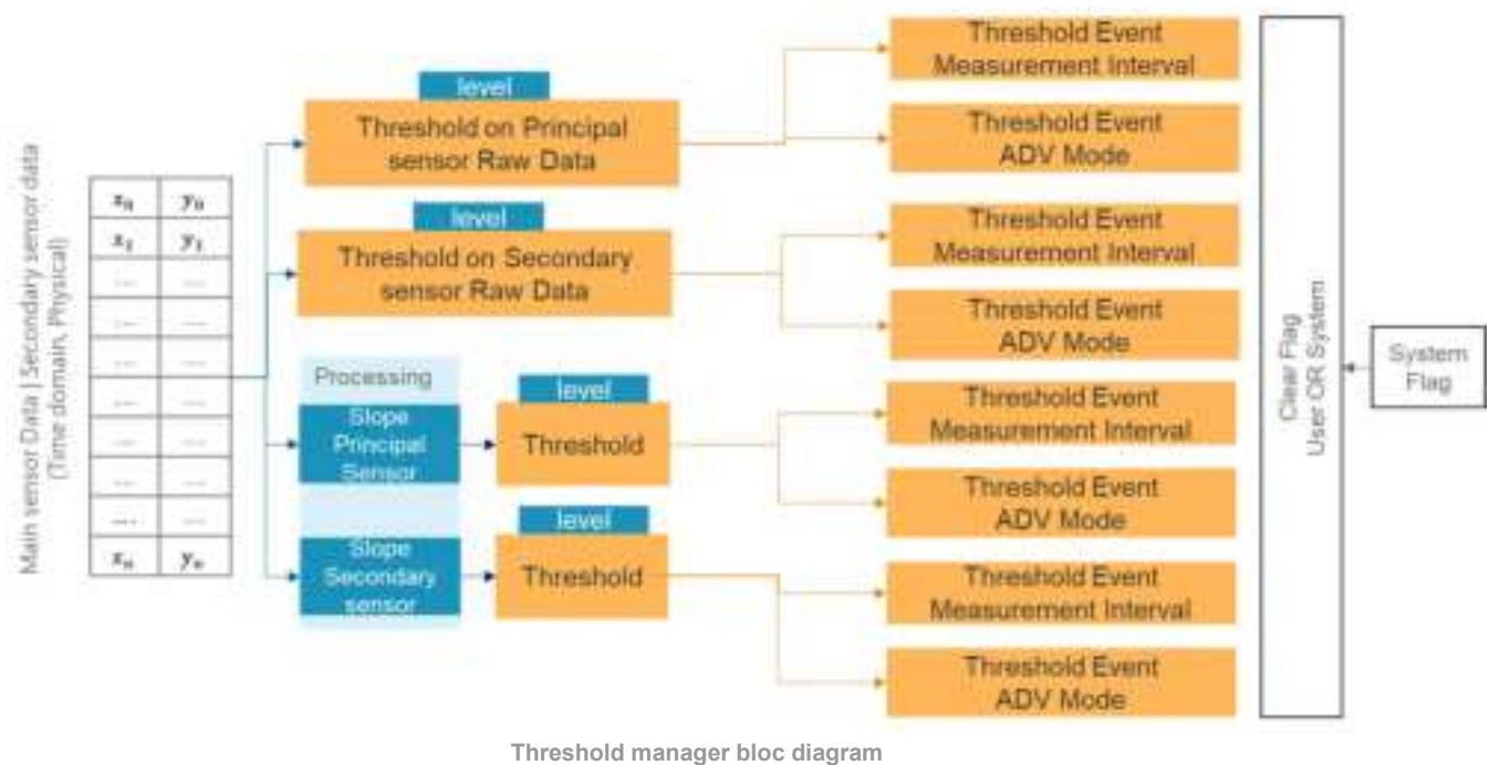
Threshold manager bloc diagram
