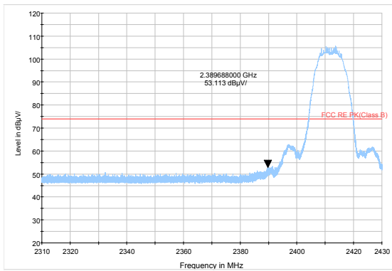
802.11b-Channel 1 Peak
