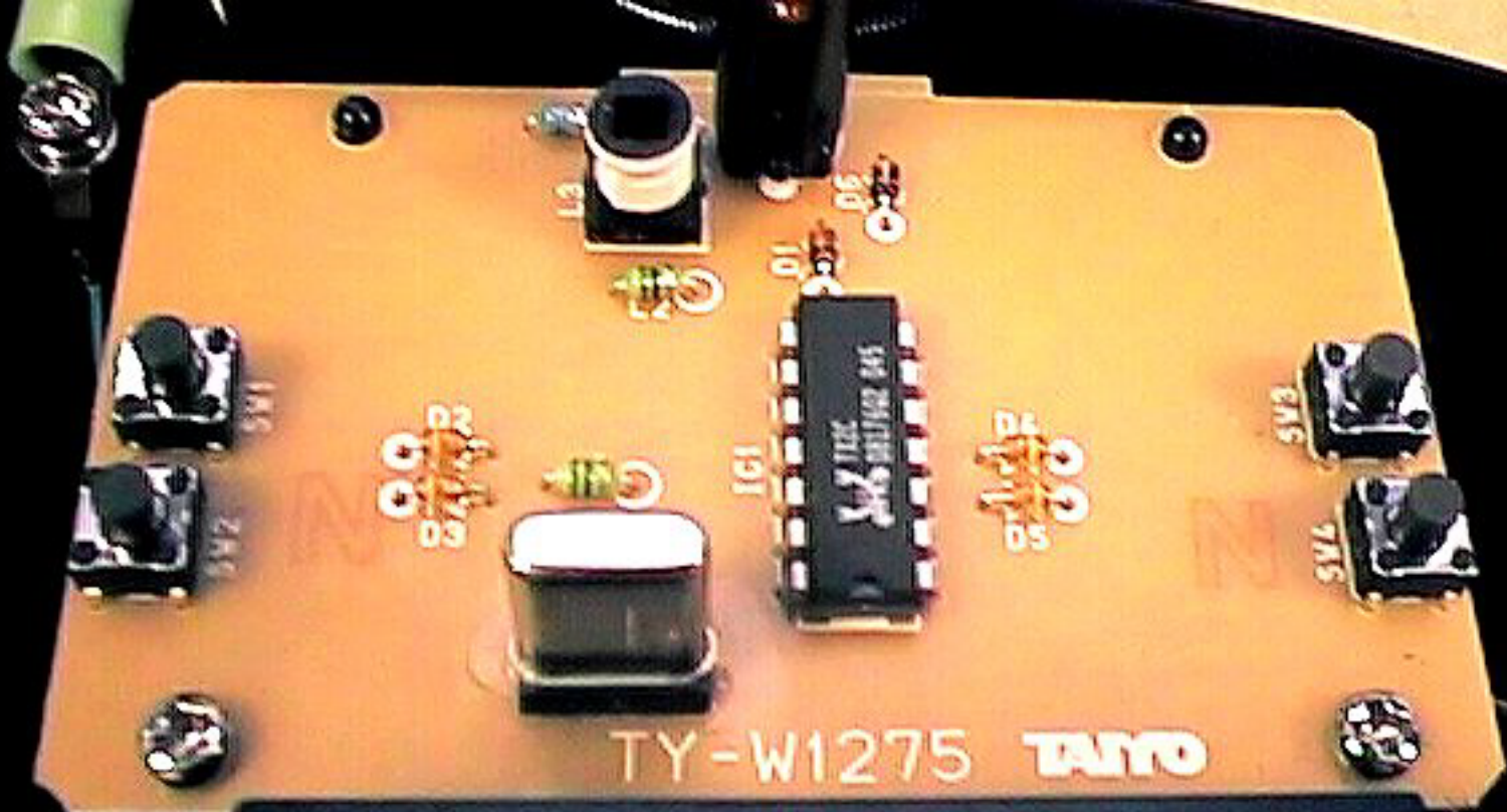
PCB Circuit Side
