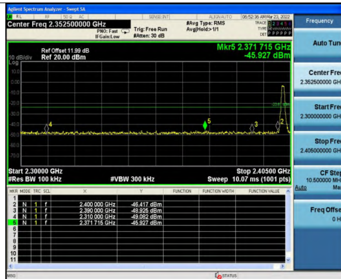
BLE_1M_Ant1_Low_2402
