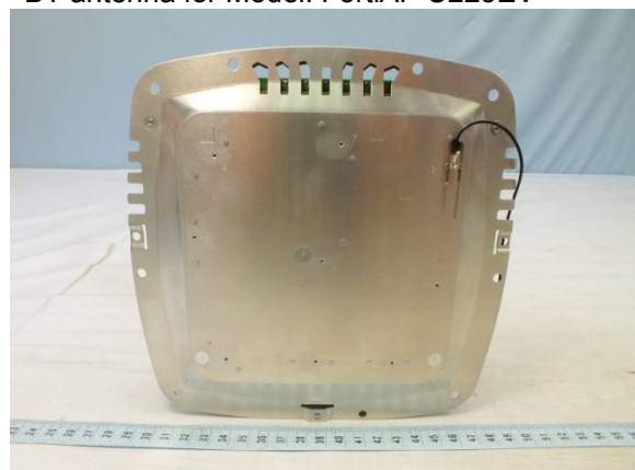
BT antenna for Model: FortiAP U223EV
