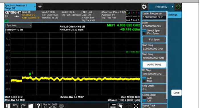
Band5-10MHz-QPSK-20600-1RB#49-3000~10000-PASS
