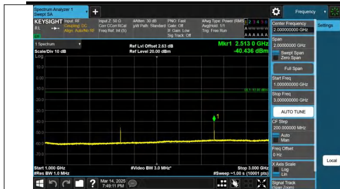
Band5-3MHz-QPSK-20525-1RB#14-1000~3000-PASS
