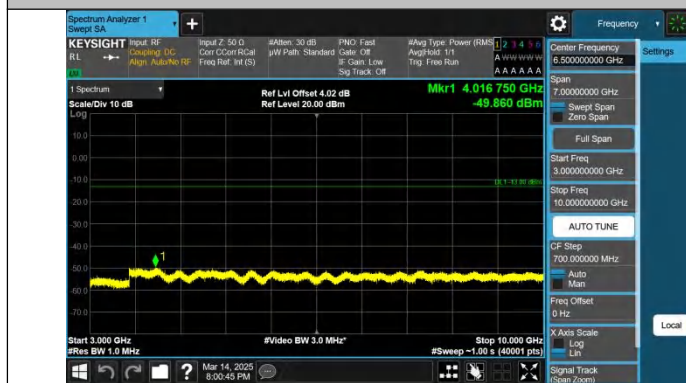
Band5-5MHz-QPSK-20625-1RB#0-3000~10000-PASS
