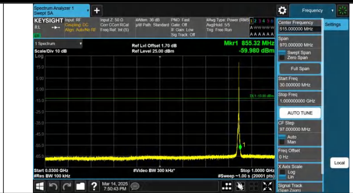
Band5-3MHz-QPSK-20635-1RB#14-30~1000-PASS
