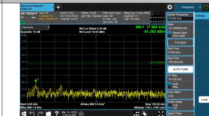
Band5-3MHz-QPSK-20635-1RB#14-0.009~0.15-PASS
