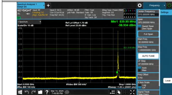
Band5-3MHz-QPSK-20635-1RB#0-30~1000-PASS
