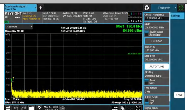
Band5-5MHz-QPSK-20525-1RB#0-0.15~30-PASS
