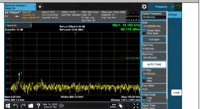
Band5-5MHz-QPSK-20625-1RB#24-0.009~0.15-PASS
