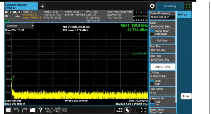
Band5-5MHz-QPSK-20625-1RB#0-0.15~30-PASS
