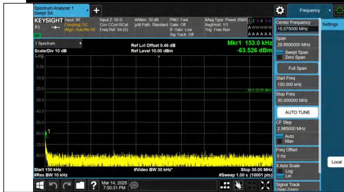
Band5-3MHz-QPSK-20635-1RB#14-0.15~30-PASS
