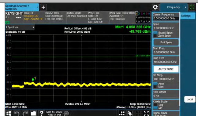
Band5-5MHz-QPSK-20425-1RB#24-3000~10000-PASS
