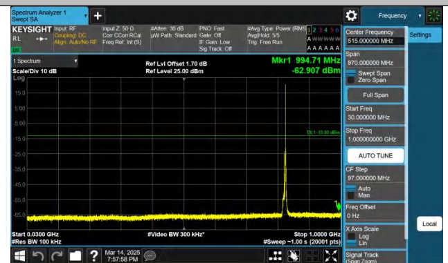
Band5-5MHz-QPSK-20425-1RB#24-30~1000-PASS
