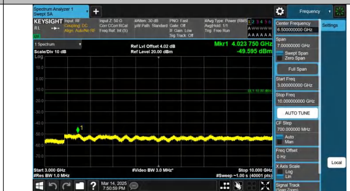
Band5-3MHz-QPSK-20635-1RB#14-3000~10000-PASS
