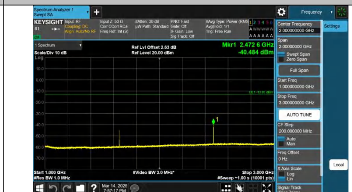
Band5-5MHz-QPSK-20425-1RB#0-1000~3000-PASS
