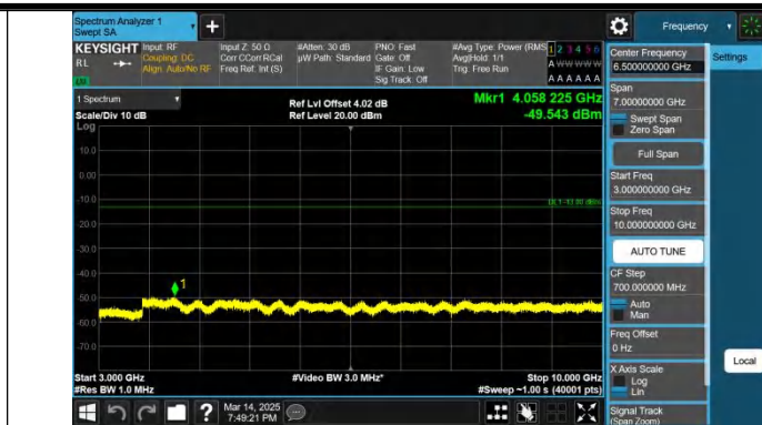
Band5-3MHz-QPSK-20525-1RB#14-3000~10000-PASS
