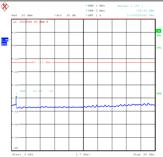
Band66_10MHz_16QAM_132622_1RB#0_3000~20000_3000~20000
