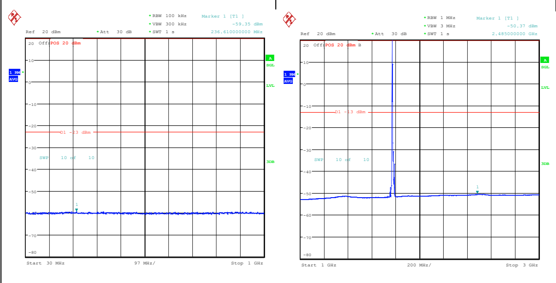
Band66_10MHz_QPSK_132622_1RB#0_30~1000_0_30~1000 Band66_10MHz_QPSK_132622_1RB#0_1000~3000_00_1000~3000
