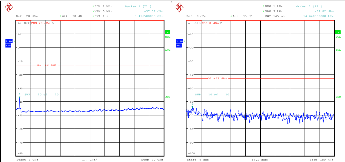
Band66_3MHz_QPSK_131987_1RB#0_3000~20000_3000~20000 Band66_3MHz_16QAM_131987_1RB#0_0.009~0.15_0.009~0.15
