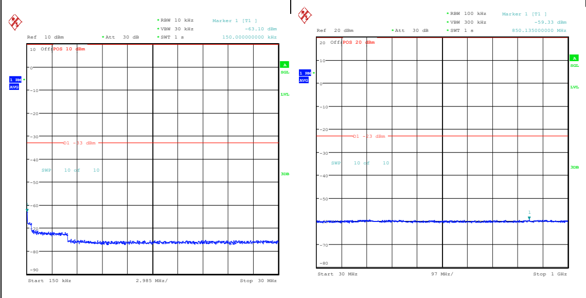
Band66_15MHz_16QAM_132322_1RB#0_0.15~30_0.15~30 Band66_15MHz_16QAM_132322_1RB#0_30~1000_30~1000
