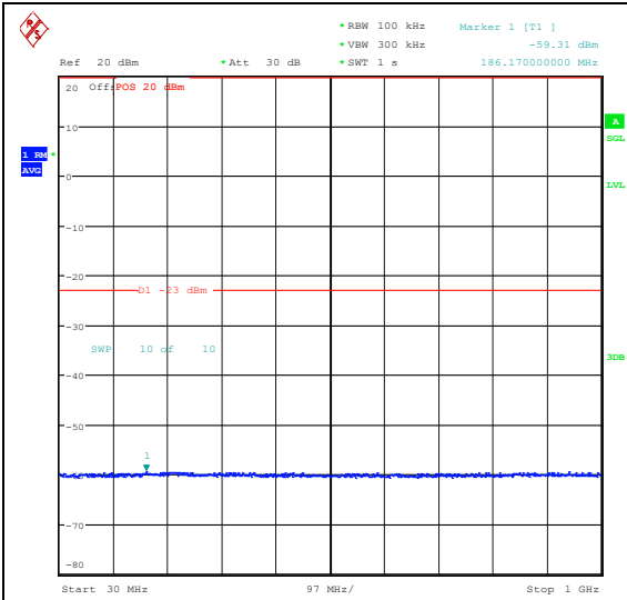
Band66_15MHz_QPSK_132597_1RB#0_30~100 0_30~1000
