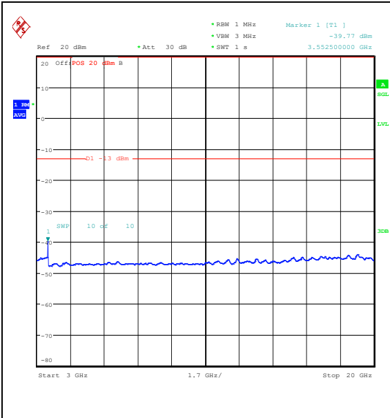
Band66_3MHz_QPSK_132657_1RB#0_3000~20000_3000~20000
