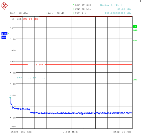
Band66_3MHz_16QAM_132657_1RB#0_3000~20000_3000~20000
