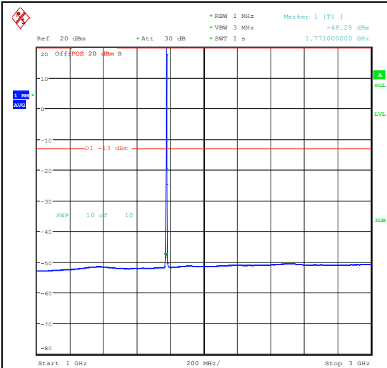
Band66_3MHz_16QAM_132657_1RB#0_1000~3000_1000~3000
