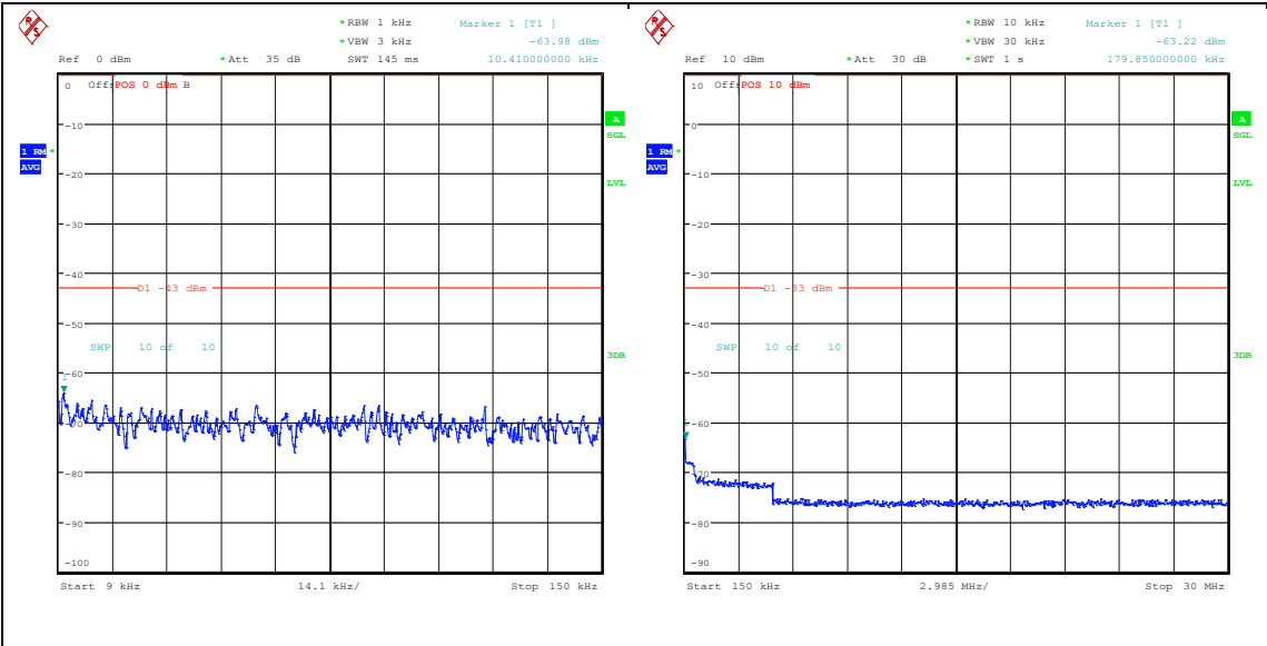
Band66_10MHz_QPSK_132622_1RB#0_0.009~0.15_0.009~0.15 Band66_10MHz_QPSK_132622_1RB#0_0.15~30_0.15~30
