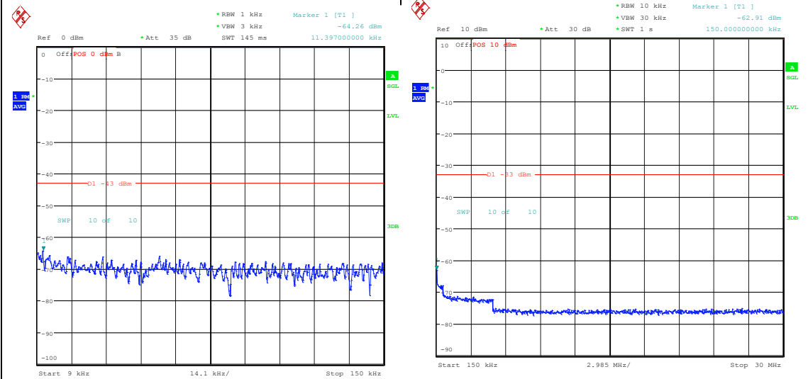
Band66_3MHz_QPSK_132322_1RB#0_0.009~0.15_0.009~0.15 Band66_3MHz_QPSK_132322_1RB#0_0.15~30_0.15~30
