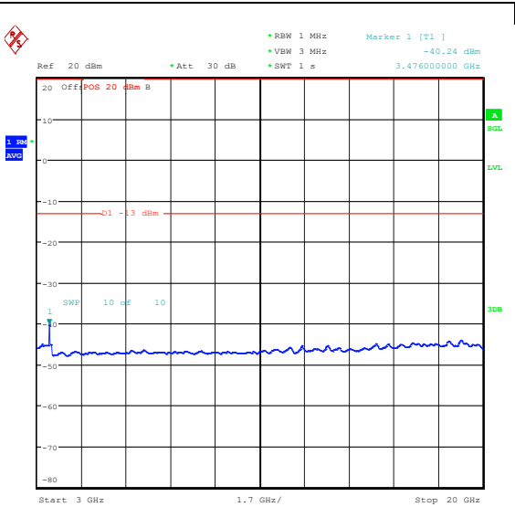
Band66_15MHz_16QAM_132322_1RB#0_3000~20000_3000~20000
