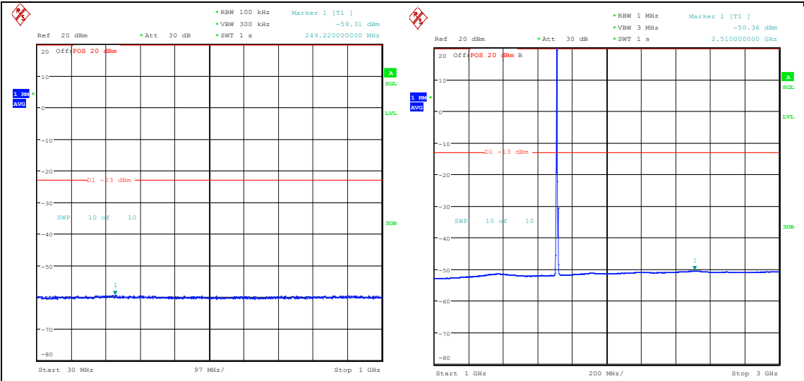
Band66_5MHz_QPSK_131997_1RB#0_30~1000_30~1000 Band66_5MHz_QPSK_131997_1RB#0_1000~3000_0_1000~3000
