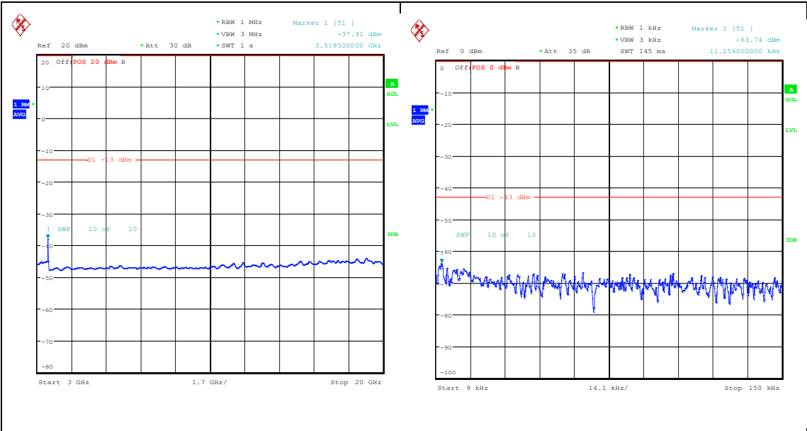
Band66_20MHz_QPSK_132572_1RB#0_3000~20000_3000~20000 Band66_20MHz_16QAM_132572_1RB#0_0.009~0.15_0.009~0.15
