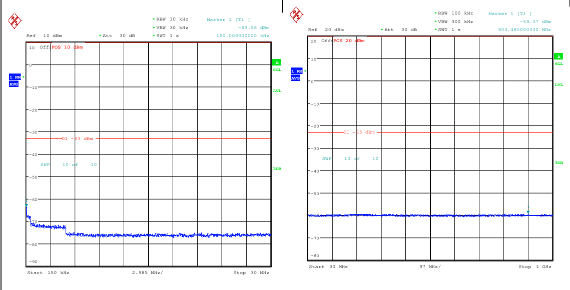
Band66_5MHz_16QAM_132322_1RB#0_0.15~30_0.15~30 Band66_5MHz_16QAM_132322_1RB#0_30~1000_30~1000
