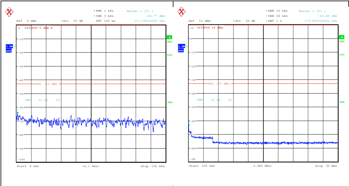
Band66_20MHz_QPSK_132072_1RB#0_0.009~0.15_0.009~0.15 Band66_20MHz_QPSK_132072_1RB#0_0.15~30_0.15~30
