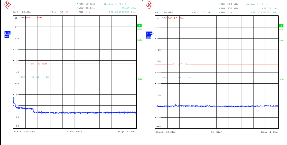
Band66_10MHz_16QAM_132022_1RB#0_0.15~30_0.15~30 Band66_10MHz_16QAM_132022_1RB#0_30~100_30~1000
