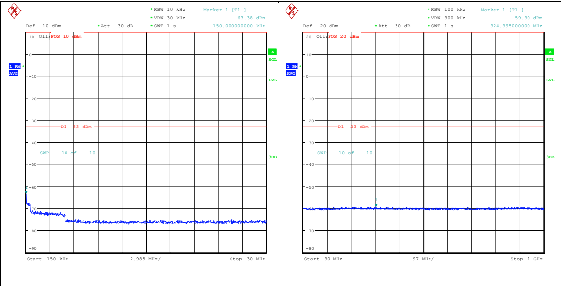
Band66_15MHz_16QAM_132597_1RB#0_0.15~30_0.15~30
