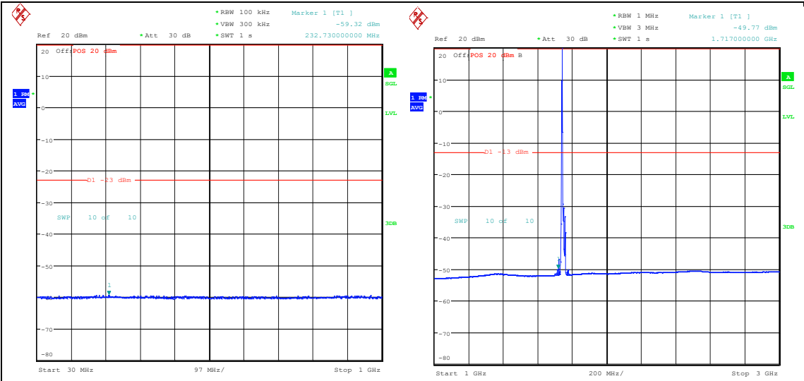
Band66_10MHz_QPSK_132322_1RB#0_30~1000_0_30~1000 Band66_10MHz_QPSK_132322_1RB#0_1000~3000_00_1000~3000
