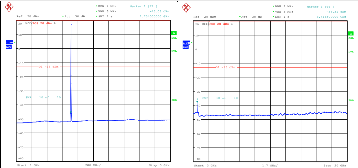
Band66_3MHz_16QAM_131987_1RB#0_1000~3000_1000~3000 Band66_3MHz_16QAM_131987_1RB#0_3000~20000_3000~20000
