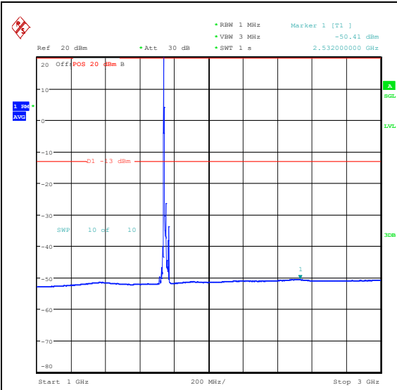
Band66_15MHz_16QAM_132322_1RB#0_1000~3000_1000~3000
