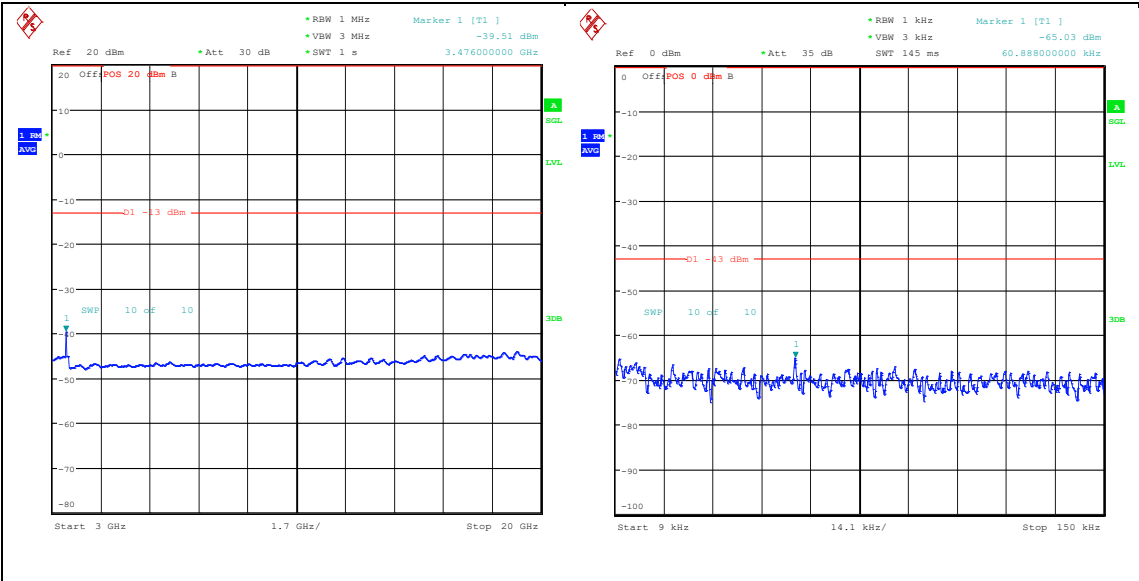
Band66_15MHz_QPSK_132322_1RB#0_3000~20000_3000~20000 Band66_15MHz_16QAM_132322_1RB#0_0.009~0.15_0.009~0.15
