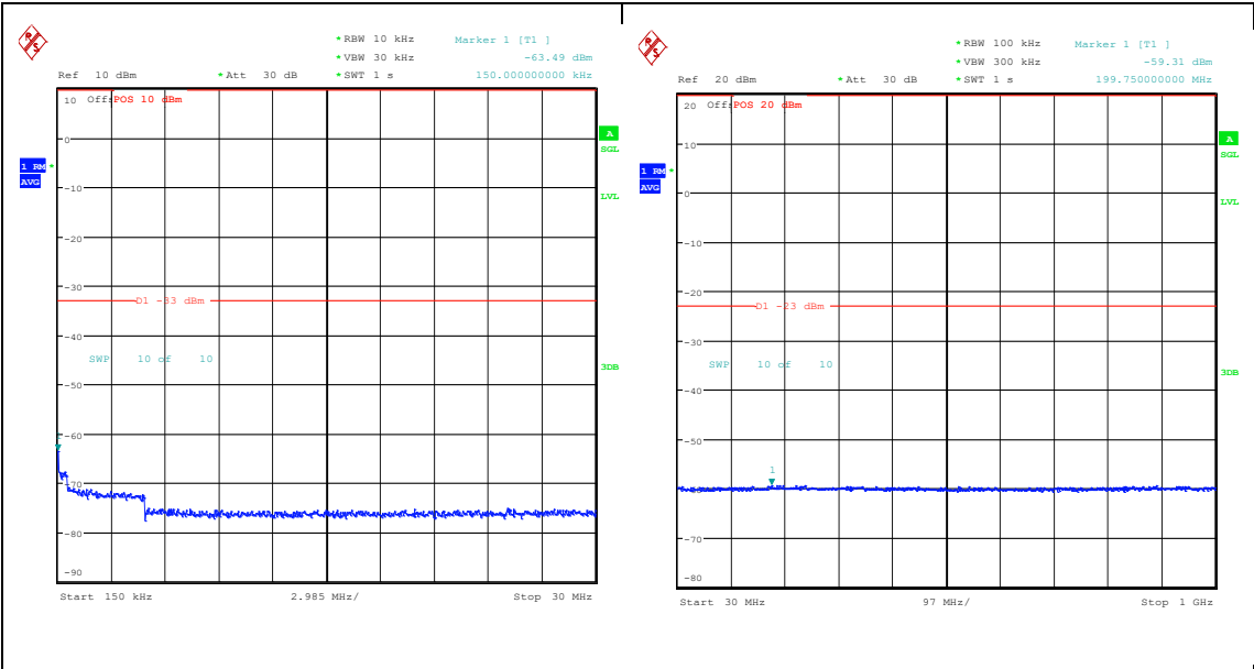
Band66_5MHz_16QAM_131997_1RB#0_0.15~30_0.15~30 Band66_5MHz_16QAM_131997_1RB#0_30~1000_30~1000
