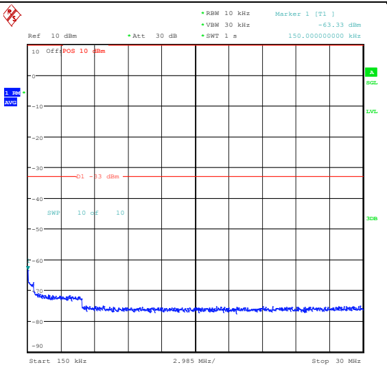
Band66_20MHz_QPSK_132572_1RB#0_0.15~30_0.15~30
