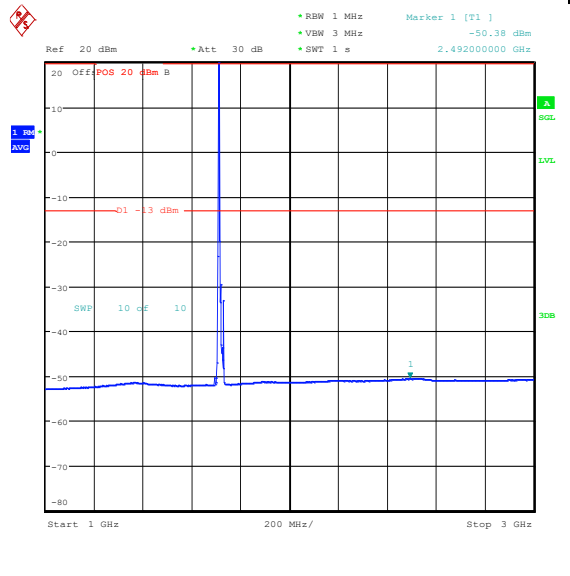
Band66_10MHz_QPSK_132022_1RB#0_1000~30_00_1000~3000
