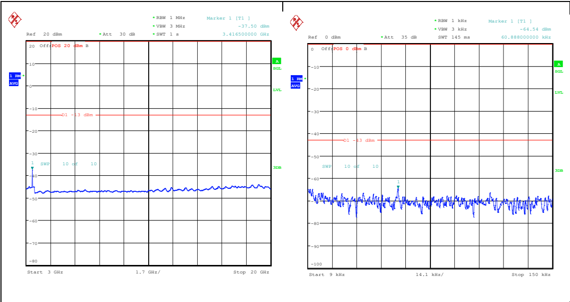
Band66_10MHz_QPSK_132022_1RB#0_3000~20000_3000~20000 Band66_10MHz_16QAM_132022_1RB#0_0.009~0.15_0.009~0.15
