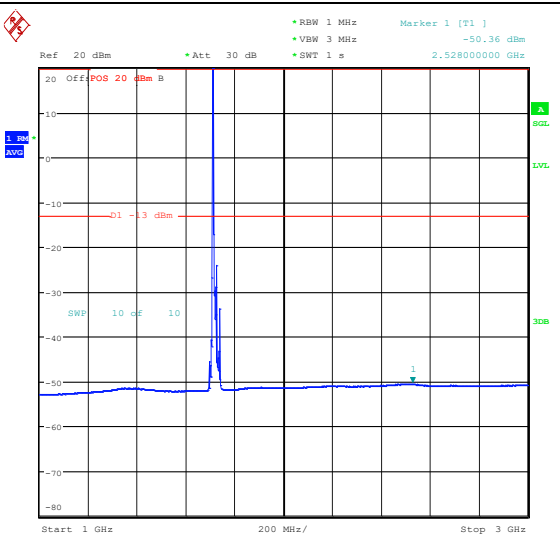
Band66_15MHz_QPSK_132047_1RB#0_1000~30 00_1000~3000
