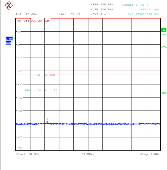
Band66_10MHz_QPSK_132022_1RB#0_30~100_0_30~1000
