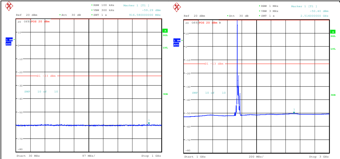
Band66_20MHz_QPSK_132322_1RB#0_30~1000_30~1000 Band66_20MHz_QPSK_132322_1RB#0_1000~3000_1000~3000
