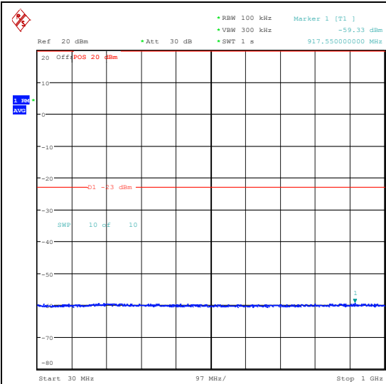
Band66_15MHz_QPSK_132047_1RB#0_30~100 0_30~1000
