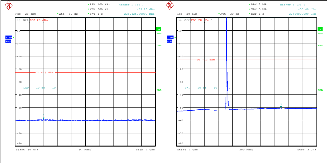
Band66_20MHz_QPSK_132072_1RB#0_30~100_0_30~1000 Band66_20MHz_QPSK_132072_1RB#0_1000~3000_00_1000~3000
