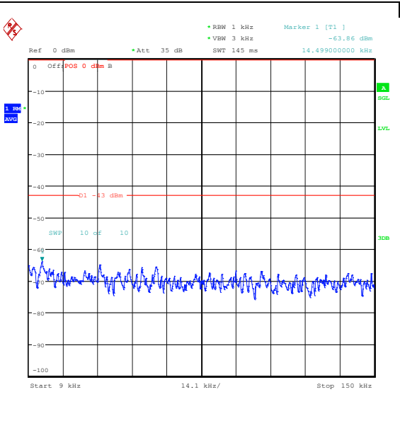
Band66_3MHz_16QAM_132657_1RB#0_0.009~0.15_0.009~0.15
