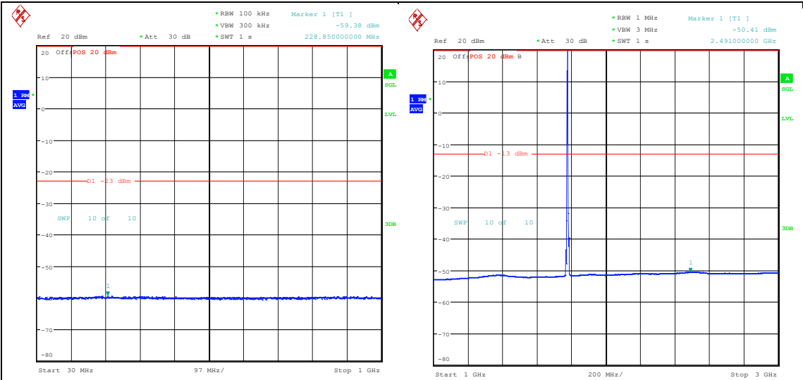
Band66_5MHz_QPSK_132647_1RB#0_30~1000_30~1000 Band66_5MHz_QPSK_132647_1RB#0_1000~3000_0_1000~3000
