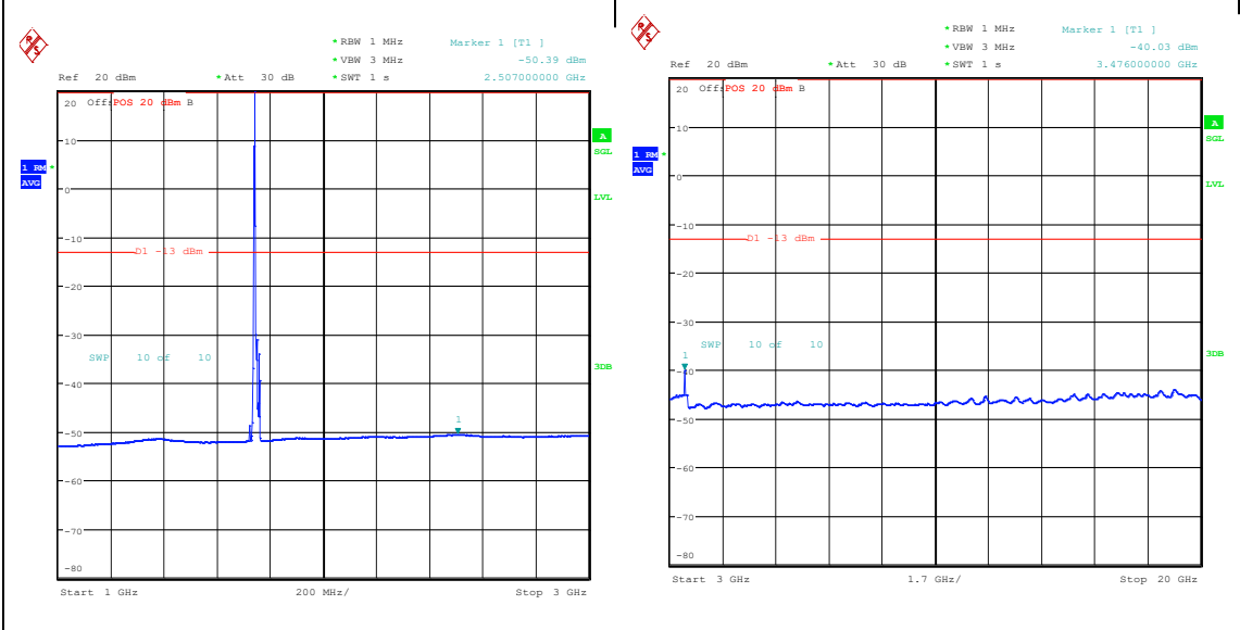
Band66_10MHz_16QAM_132322_1RB#0_1000~3000_1000~3000 Band66_10MHz_16QAM_132322_1RB#0_3000~20000_0000_3000~20000
