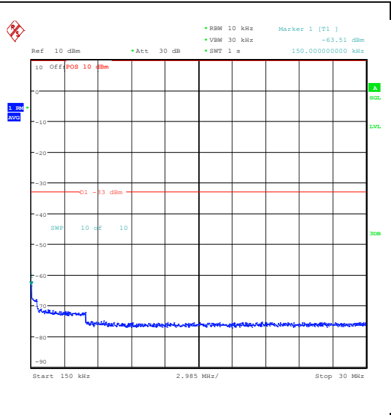
Band66_10MHz_QPSK_132022_1RB#0_0.15~30_0.15~30
