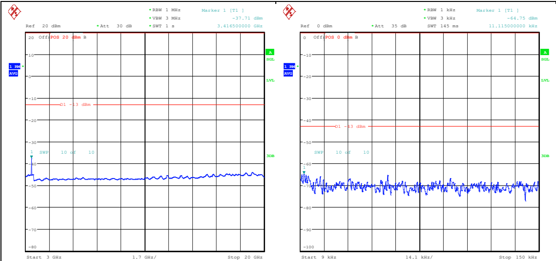
Band66_20MHz_QPSK_132072_1RB#0_3000~20000_3000~20000 Band66_20MHz_16QAM_132072_1RB#0_0.009~0.15_0.009~0.15
