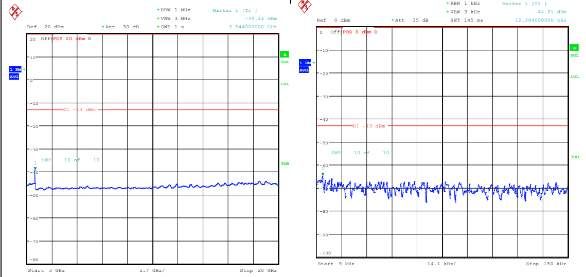
Band66_5MHz_QPSK_132647_1RB#0_3000~20000_000_3000~20000 Band66_5MHz_16QAM_132647_1RB#0_0.009~0.15_0.009~0.15
