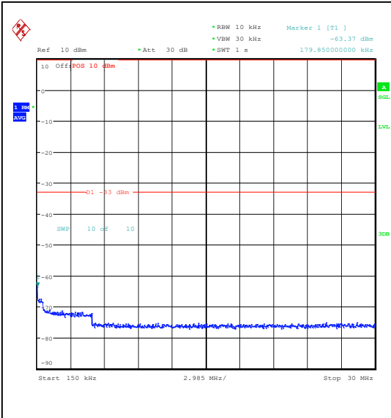
Band66_15MHz_16QAM_132047_1RB#0_0.15~30_0.15~30
