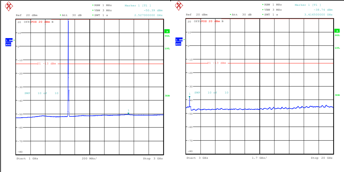
Band66_5MHz_16QAM_131997_1RB#0_1000~3000_1000~3000 Band66_5MHz_16QAM_131997_1RB#0_3000~20000_3000~20000
