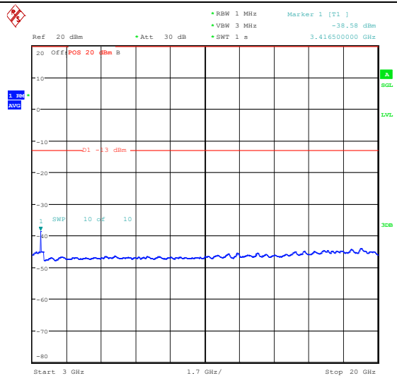
Band66_10MHz_16QAM_132022_1RB#0_3000~20000_3000~20000
