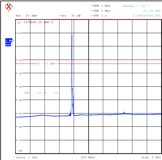
Band66_10MHz_16QAM_132622_1RB#0_1000~3000_1000~3000
