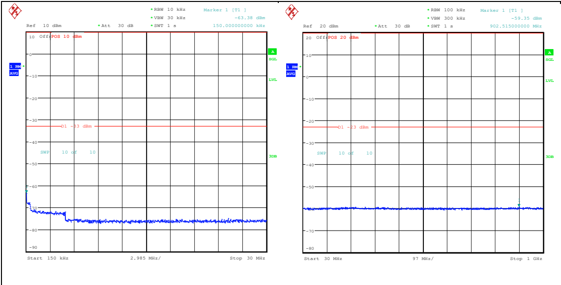
Band66_10MHz_16QAM_132322_1RB#0_0.15~30_0.15~30 Band66_10MHz_16QAM_132322_1RB#0_30~100_0_30~1000
