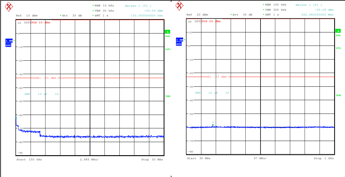
Band66_20MHz_16QAM_132572_1RB#0_0.15~30_0.15~30 Band66_20MHz_16QAM_132572_1RB#0_30~100_30~1000
