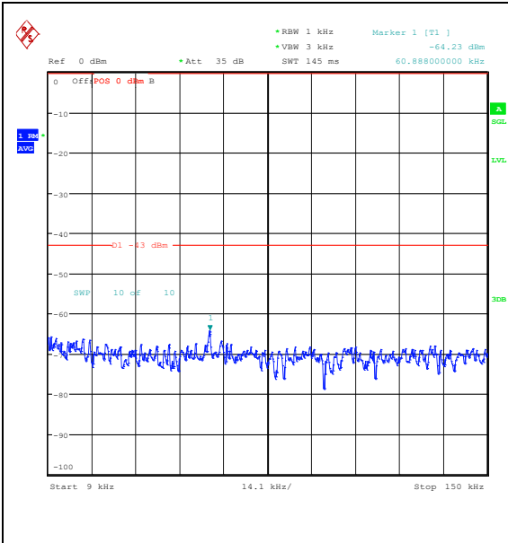
Band66_10MHz_QPSK_132022_1RB#0_0.009~0.15_0.009~0.15
