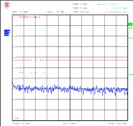
Band66_15MHz_16QAM_132322_1RB#0_1000~3000_1000~3000
