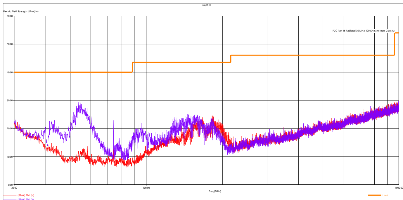
Figure 5 - Radiated Emissions Plot, GFSK
