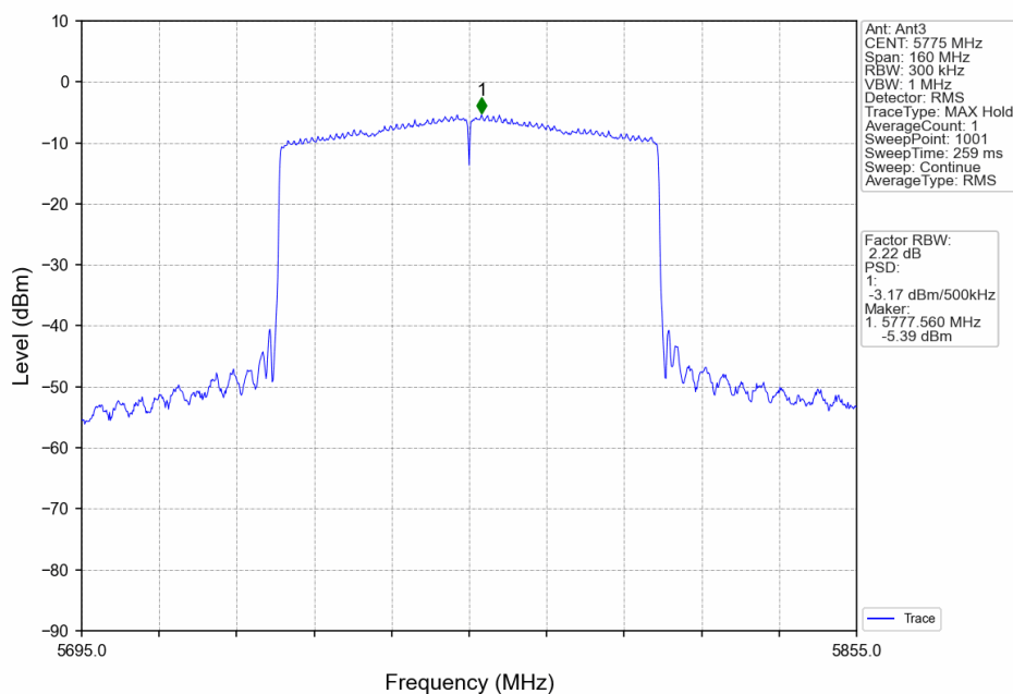
802.11ax(HEW80)_MCH_5775MHz_RU996_Left_Ant3_NTNV
