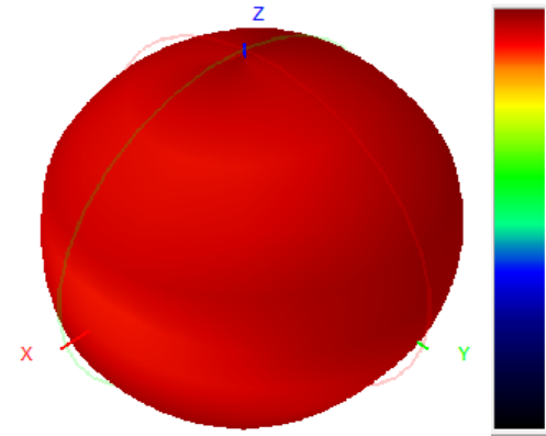
903.0MHz H+V, Eff: 10.2%
