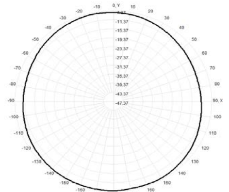
Total(H-XY), Max= -7.86dBi, CirD=4.30
