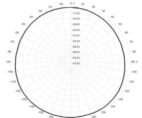
Total(H-XY), Max= -7.95dBi, CirD=4.19
