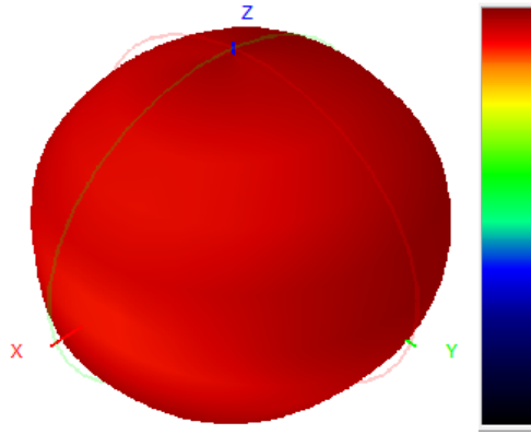
921.0MHz H+V, Eff: 11.6%
