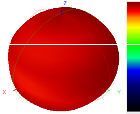
922.0MHz H+V, Eff: 11.6%
