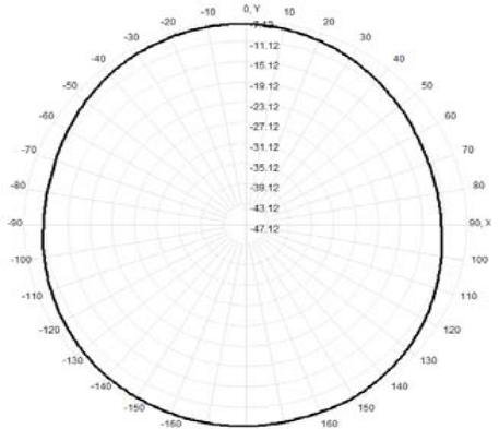
Total(H-XY), Max= -7.54dBi, CirD=4.64
