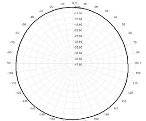
Total(H-XY), Max= -8.02dBi, CirD=4.23
