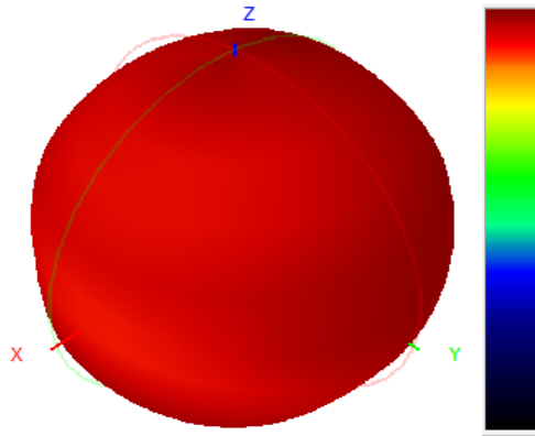
923.0MHz H+V, Eff: 11.7%
