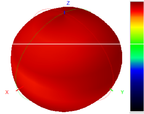
904.0MHz H+V, Eff: 10.2%
