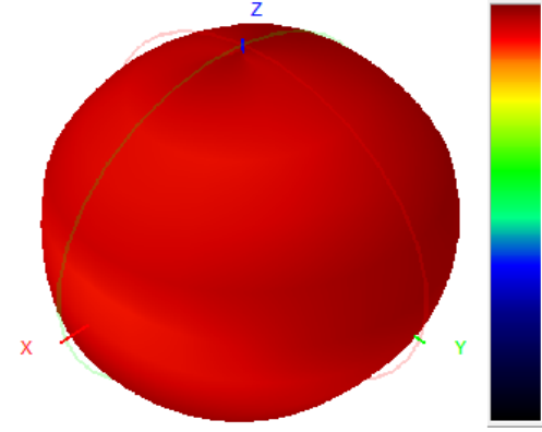
905.0MHz H+V, Eff: 10.3%
