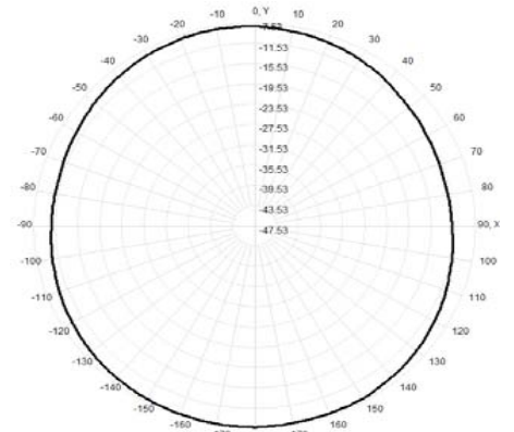
Total(H-XY), Max= -7.94dBi, CirD=4.24
