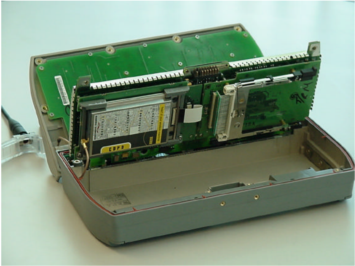
Figure 6: Modem with interface board integrated into the T5200
