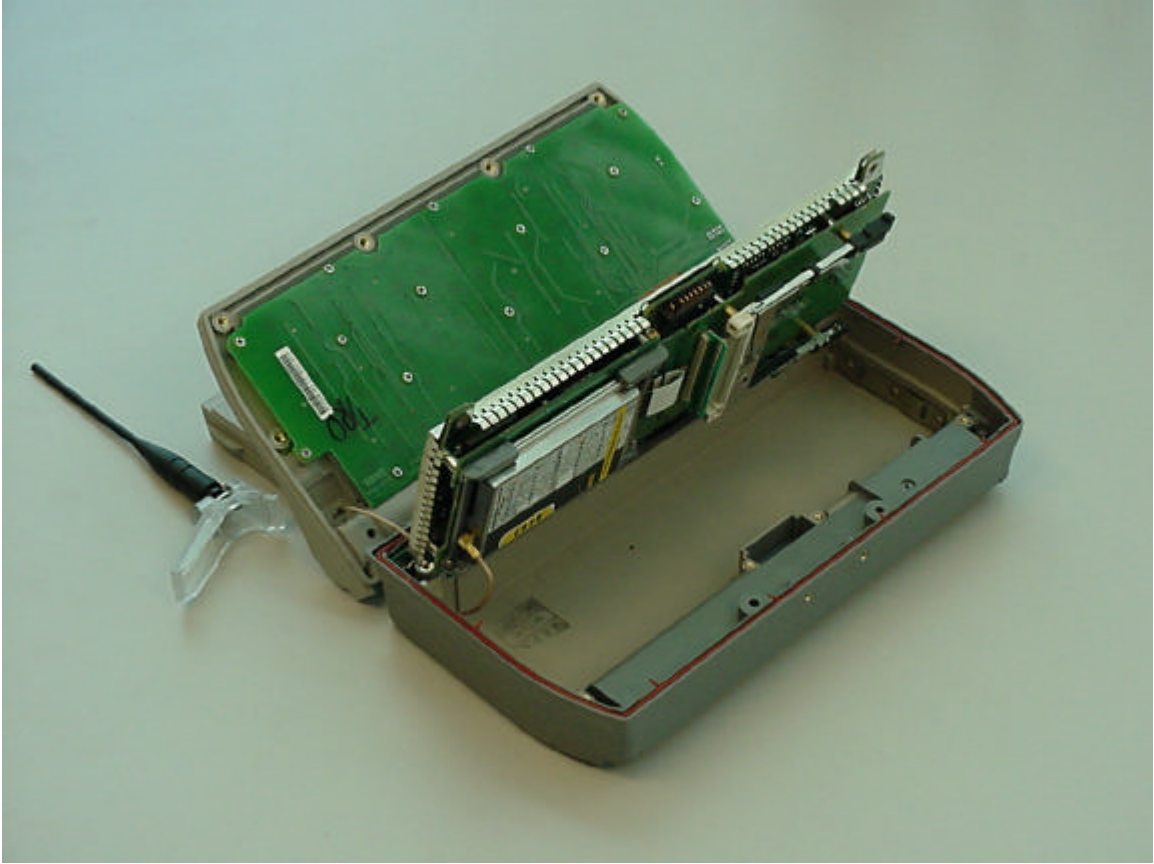
Figure 5: Modem with interface board integrated into the T5200
