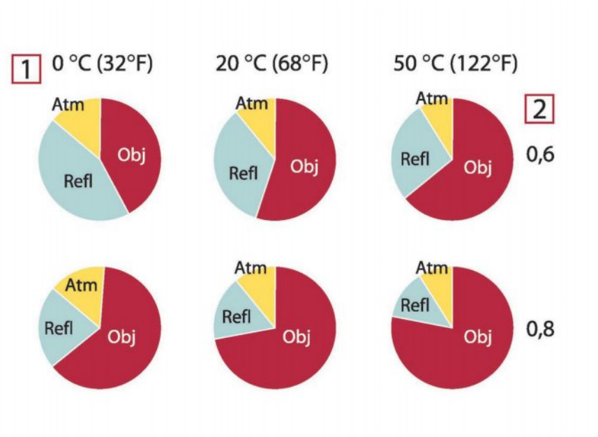
Figure 33.3 Relative magnitudes of radiation sources under varying measurement conditions (LW camera). 1: Object temperature; 2: Emittance; Obj: Object radiation; Refl: Reflected radiation; Atm: atmosphere radiation. Fixed parameters: \tau = 0.88 ; T_{\text{refl}} = 20^{\circ}\text{C} (+68°F); T_{\text{atm}} = 20^{\circ}\text{C} (+68°F).
