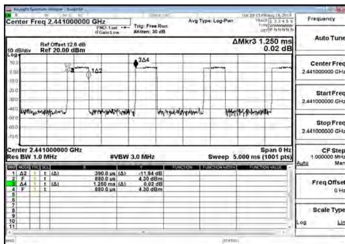
Dwell Time_π/4DQPSK_2M_DH3_2441MHz
