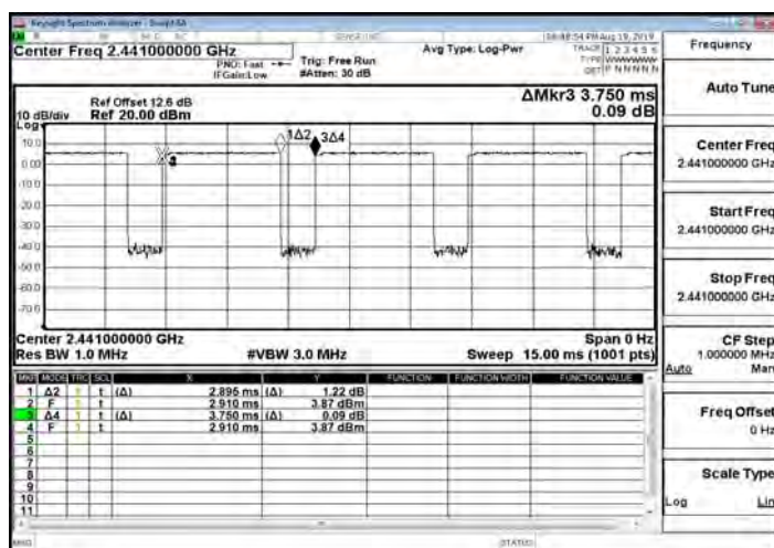
Dwell Time_π/4DQPSK_2M_DH5_2441MHz
