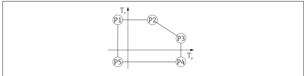
13 Aluminum housing material; process temperature range: -40 to +130 °C ( -40 to +266 °F)
