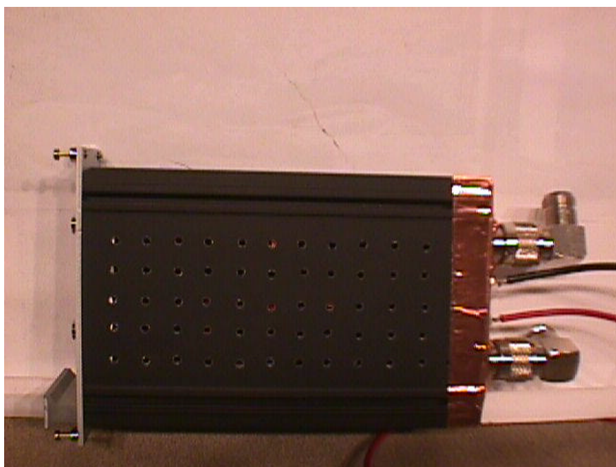
Figure 28: Amplifier, front
