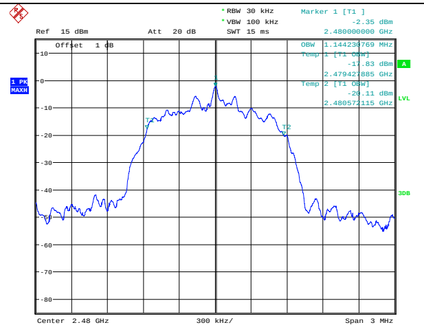
8-DPSK Mode 2480MHz
