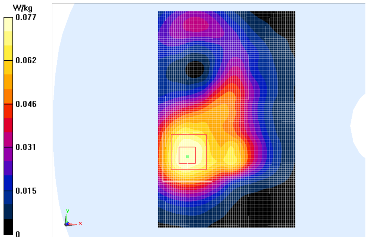
Fig.6 2450 MHz CH1
