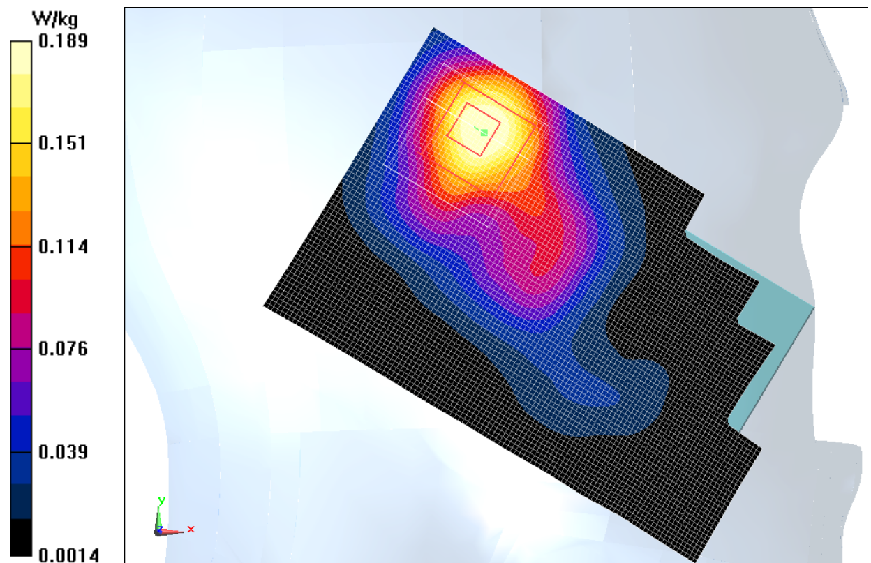
Fig.5 2450 MHz CH1
