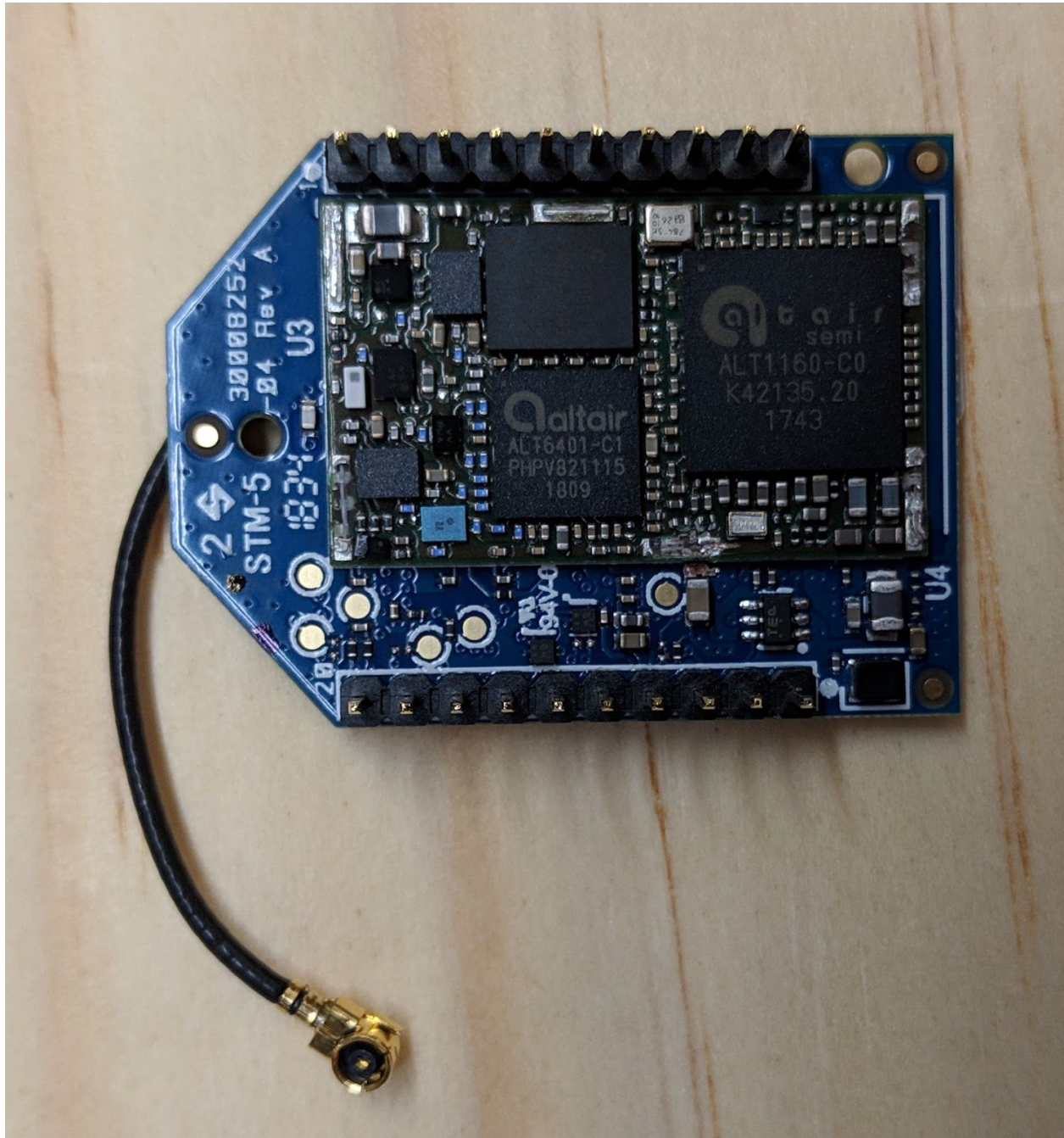
LTE Daughterboard Bottom Side
