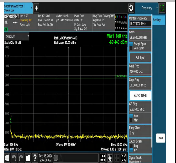
Band12_10MHz_QPSK_23095_1RB#0_0.15~30_0.15~30
