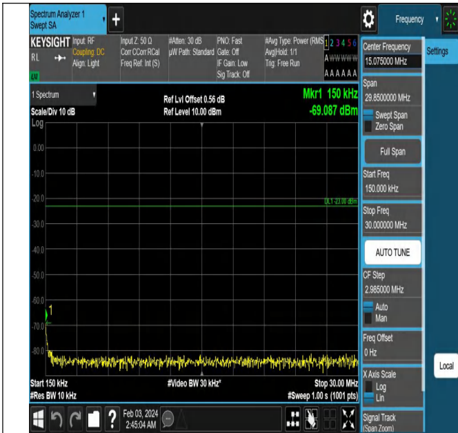
Band12_10MHz_QPSK_23130_1RB#0_0.15~30_0.15~30
