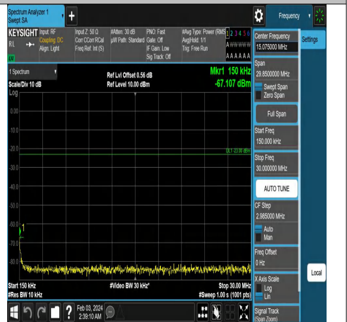
Band12_5MHz_QPSK_23035_1RB#0_0.15~30_0.15~30
