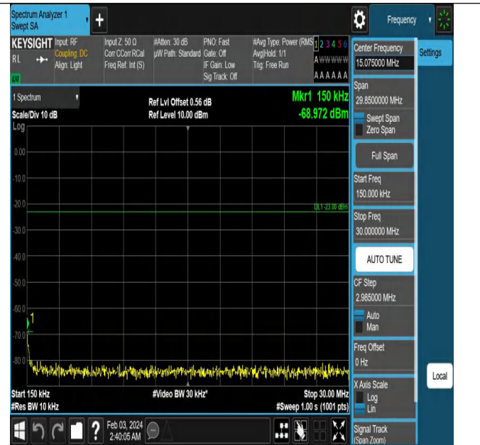
Band12_5MHz_QPSK_23155_1RB#0_0.15~30_0.15~30
