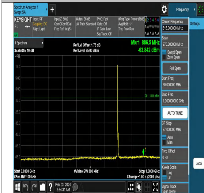
Band12_3MHz_QPSK_23095_1RB#0_30~1000_30~1000
