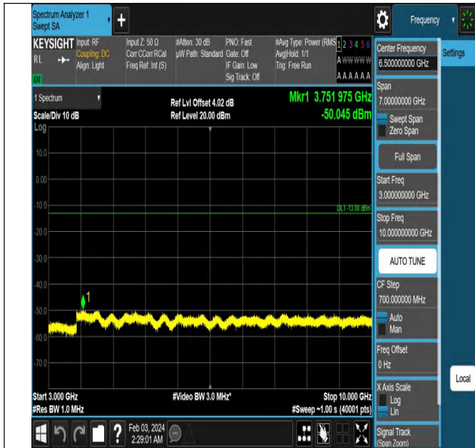
Band12_1.4MHz_QPSK_23017_1RB#0_3000~10000_3000~10000
