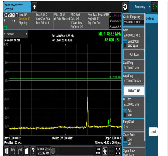
Band12_5MHz_QPSK_23095_1RB#0_30~1000_30~1000
