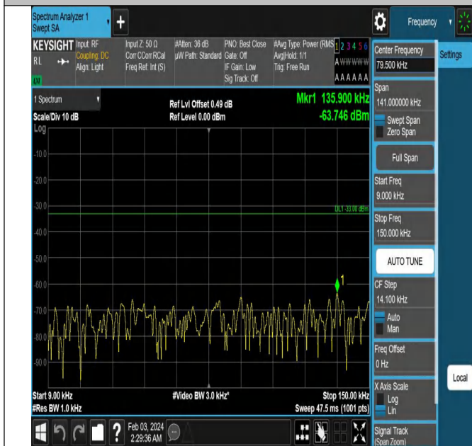
Band12_1.4MHz_QPSK_23173_1RB#0_0.009~0.15_0.009~0.
