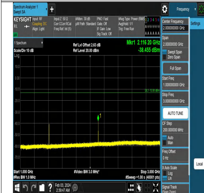
Band12_5MHz_QPSK_23095_1RB#0_1000~3000_1000~300
