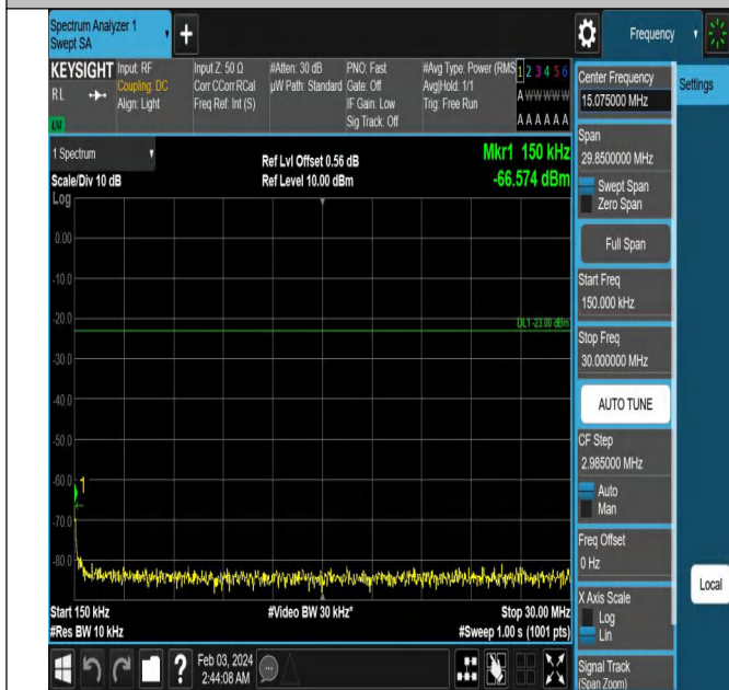
Band12_10MHz_QPSK_23060_1RB#0_0.15~30_0.15~30
