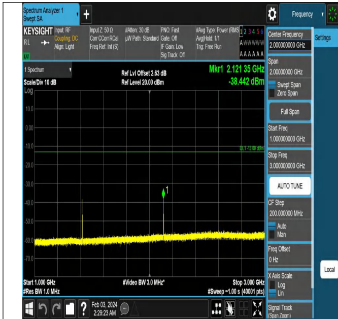
Band12_1.4MHz_QPSK_23095_1RB#0_1000~3000_1000~30
