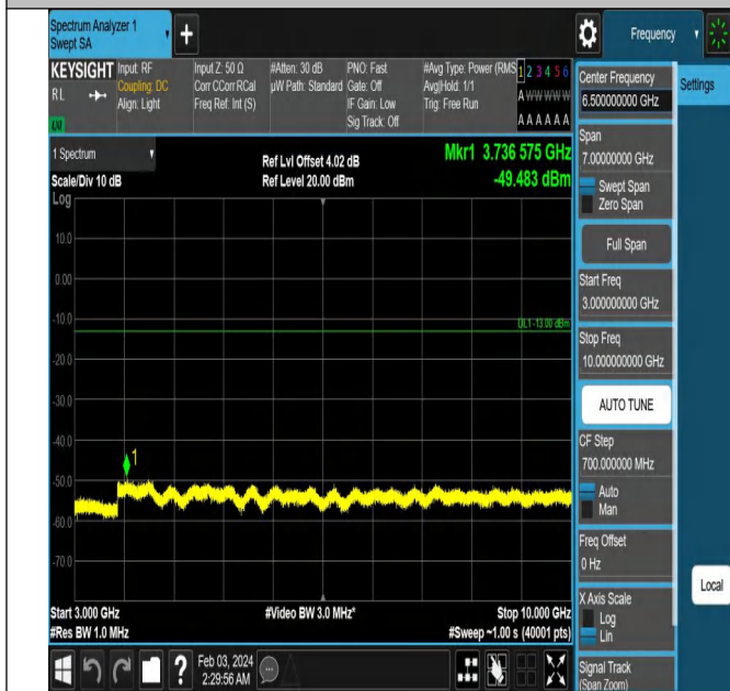
Band12_1.4MHz_QPSK_23173_1RB#0_3000~10000_3000~10000 0000
