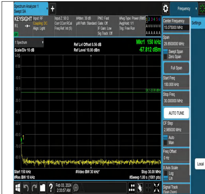
Band12_3MHz_QPSK_23025_1RB#0_0.15~30_0.15~30
