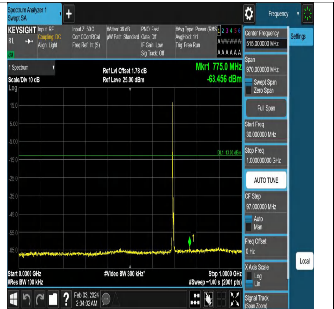
Band12_3MHz_QPSK_23025_1RB#0_30~1000_30~1000
