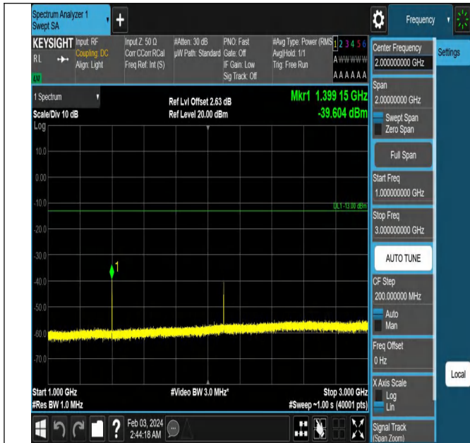
Band12_10MHz_QPSK_23060_1RB#0_1000~3000_1000~30
