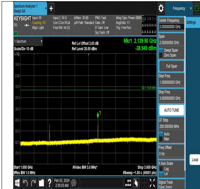
Band12_3MHz_QPSK_23165_1RB#0_1000~3000_1000~300
