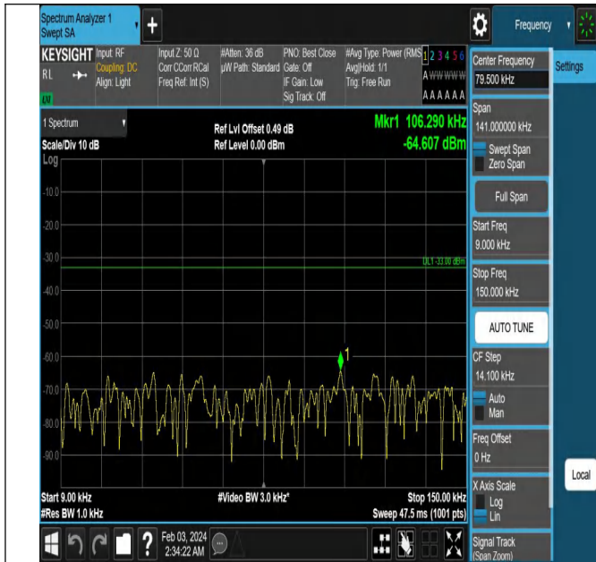
Band12_3MHz_QPSK_23095_1RB#0_0.009~0.15_0.009~0.1
