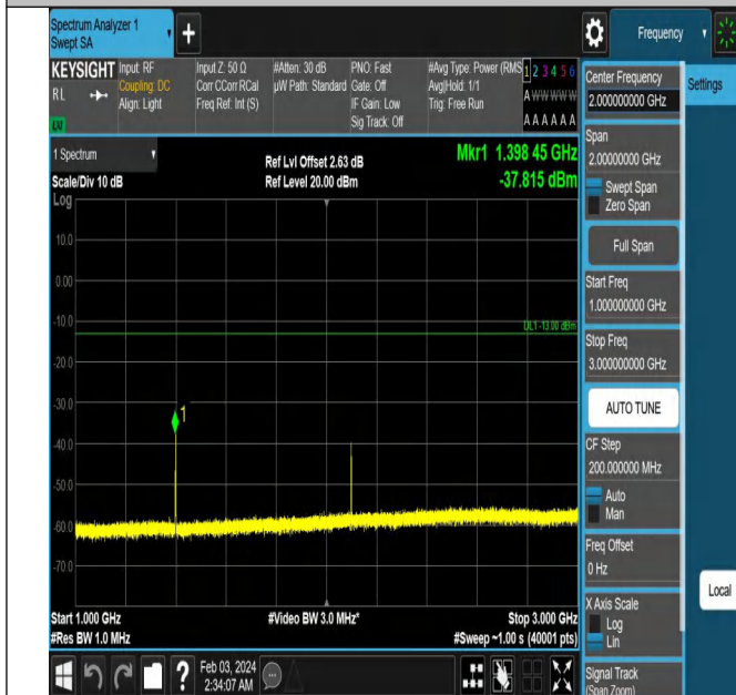
Band12_3MHz_QPSK_23025_1RB#0_1000~3000_1000~300
