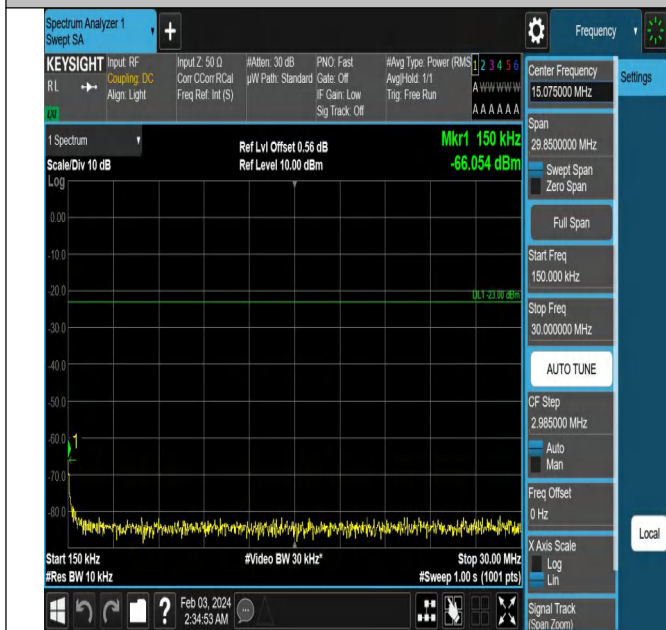
Band12_3MHz_QPSK_23165_1RB#0_0.15~30_0.15~30
