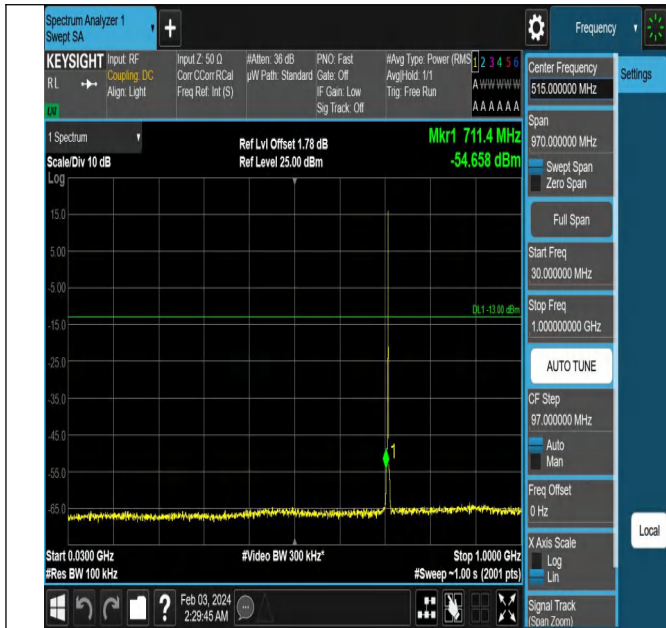
Band12_1.4MHz_QPSK_23173_1RB#0_30~1000_30~1000
