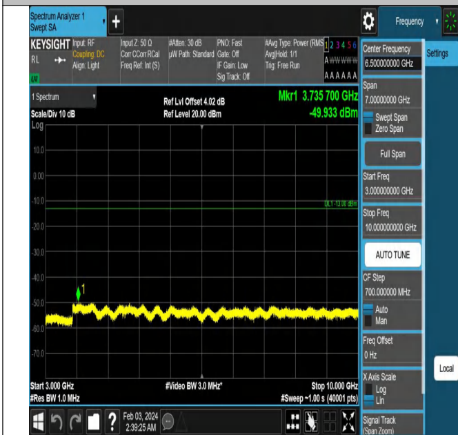
Band12_5MHz_QPSK_23035_1RB#0_3000~10000_3000~10
