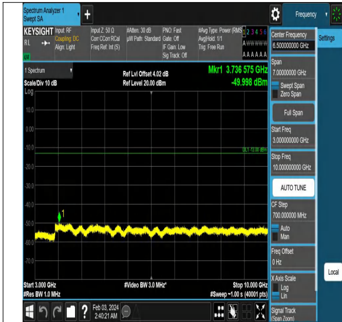
Band12_5MHz_QPSK_23155_1RB#0_3000~10000_3000~10000
