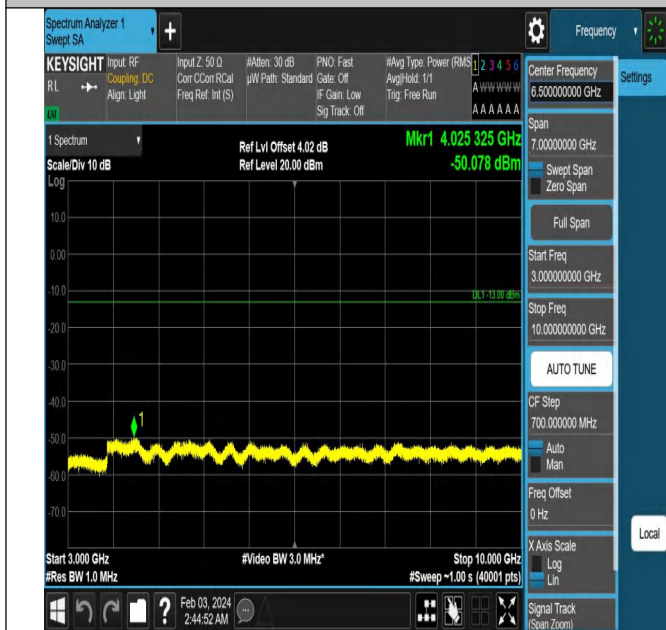
Band12_10MHz_QPSK_23095_1RB#0_3000~10000_3000~10000
