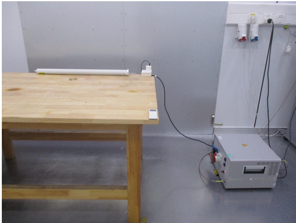
Conduction Emission
