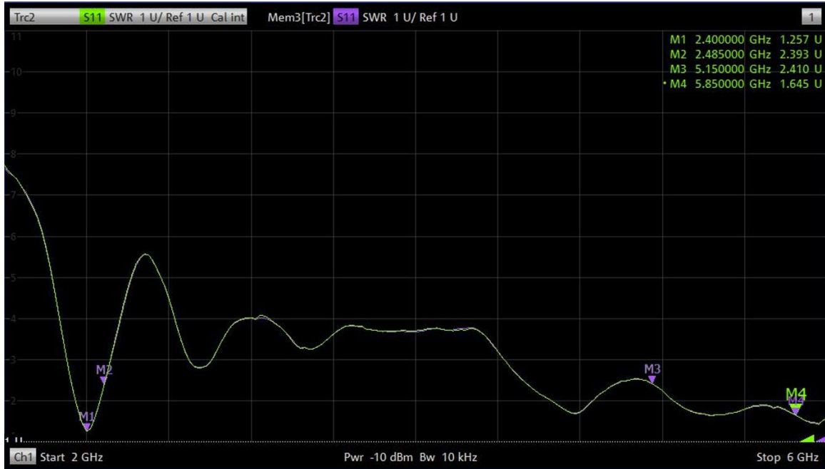
WiFi Antenna
