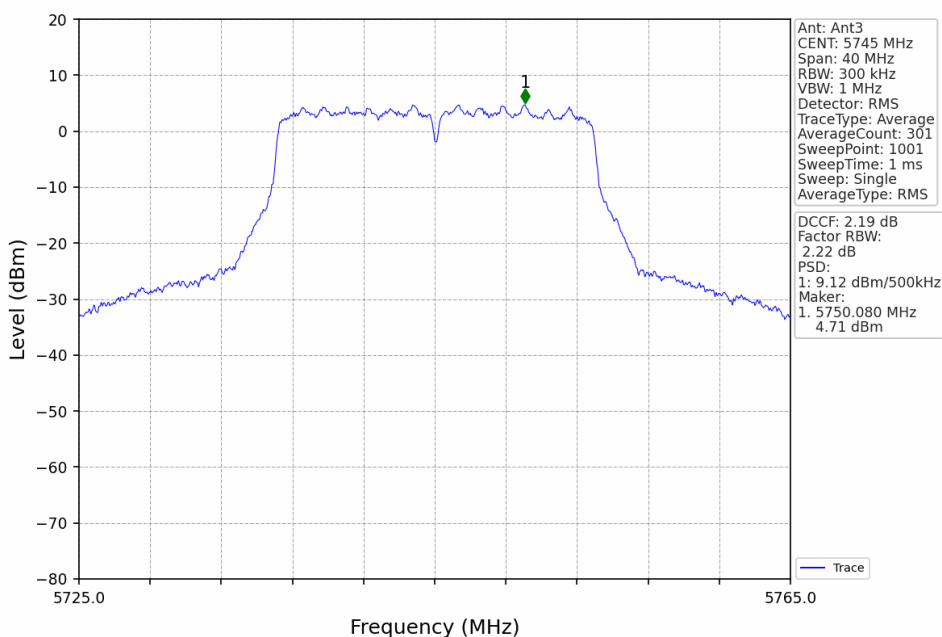
802.11n(HT20)_LCH_5745MHz_Ant3_NTNV
