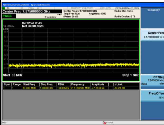
CSE_4G_B43_16QAM_5M CH45090 1RB@0
