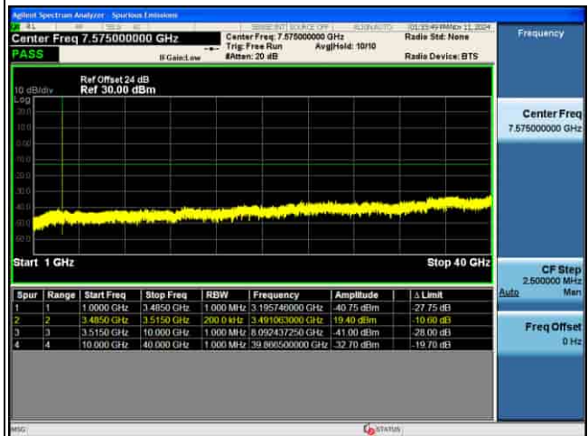
CSE_4G_B42_64QAM_20M CH42990 1RB@0_
