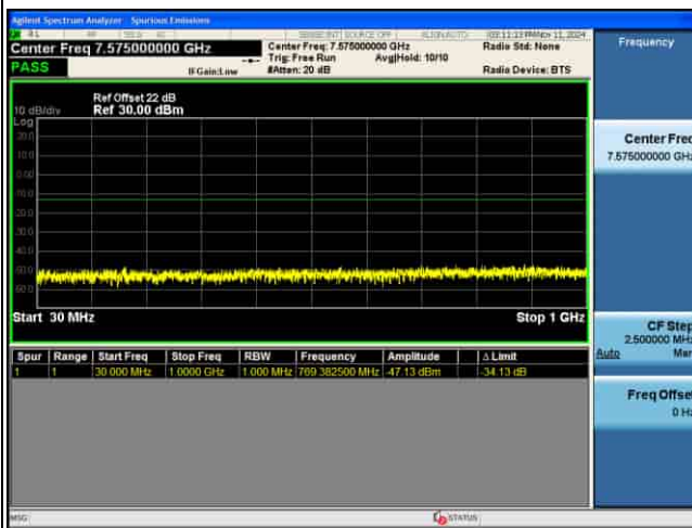
CSE_4G_B43_256QAM_10M CH45090 1RB@0
