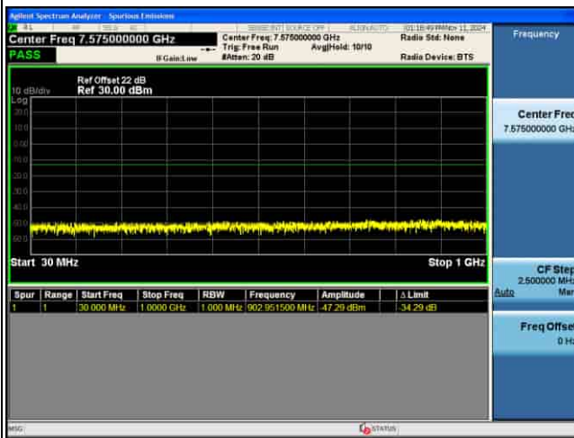
CSE_4G_B42_64QAM_15M CH42590 1RB@0
