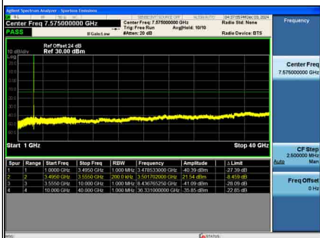
CSE_5G_n77(K)_30KHz_.PI2-BPSK_50M CH635000_1RB@1_
