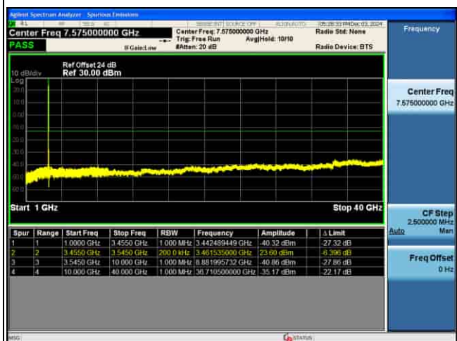
CSE_5G_n77(K)_30KHz_.PI2-BPSK_80M CH634000_1RB@1_
