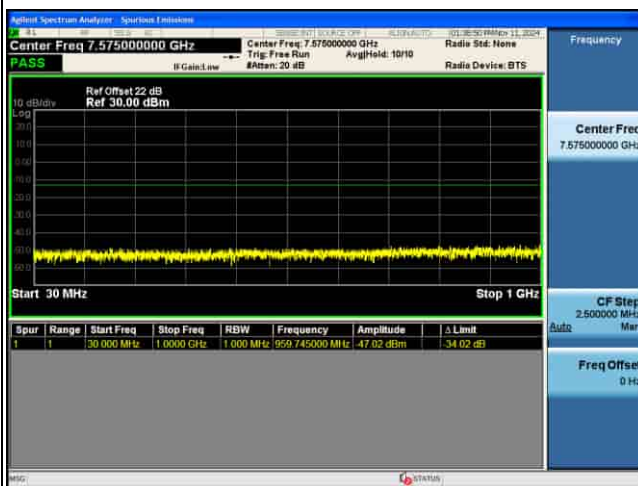
CSE_4G_B42_16QAM_20M CH42990 1RB@0
