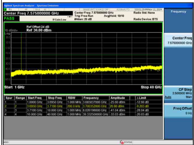
CSE_4G_B43_64QAM_5M CH45090 1RB@0_
