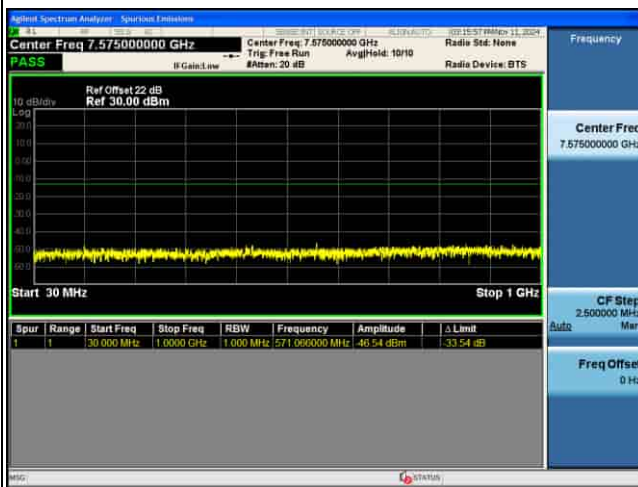
CSE_4G_B43_64QAM_10M CH45090 1RB@0
