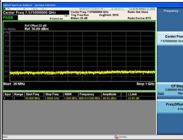
CSE_4G_B42_256QAM_10M CH42590 1RB@0
