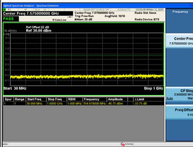
CSE_4G_B43_16QAM_15M CH45090 1RB@0
