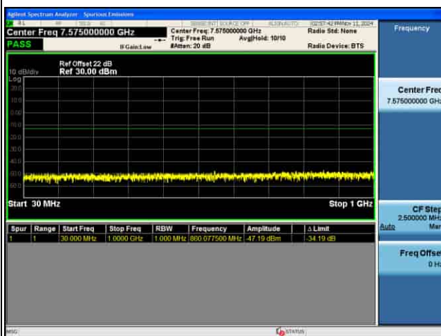
CSE_4G_B43_16QAM_5M CH45565 1RB@0
