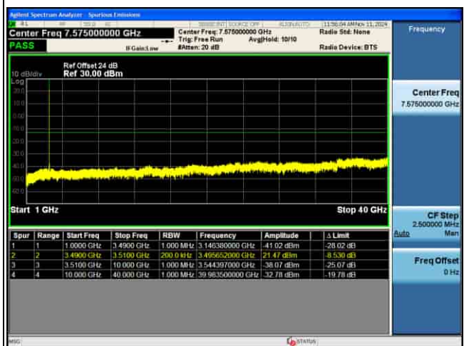
CSE_4G_B42_.QPSK_10M CH43040 1RB@0_
