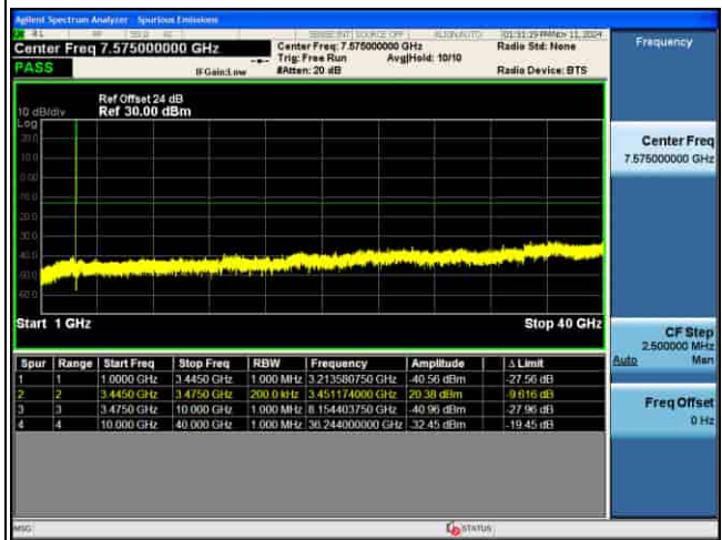
CSE_4G_B42_64QAM_20M CH42590 1RB@0_
