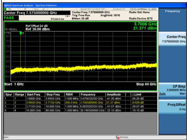
CSE_4G_B43_.QPSK_10M CH45090 1RB@0_
