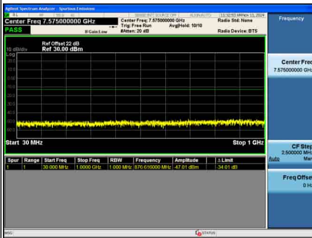
CSE_4G_B42_256QAM_5M CH42590 1RB@0
