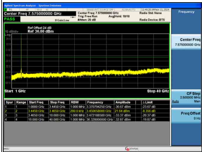
CSE_4G_B42_16QAM_10M CH42590 1RB@0_
