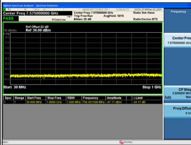
CSE_5G_n77(K)_30KHz_.PI2-BPSK_40M CH633334_1RB@1
