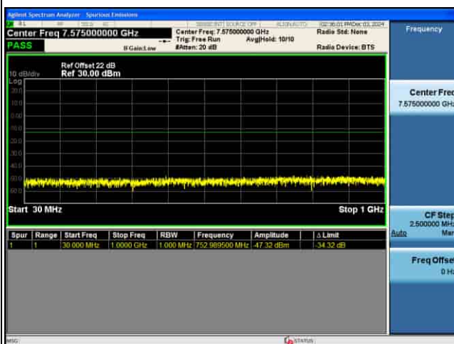
CSE_5G_n77(K)_30KHz_.PI2-BPSK_20M CH636000_1RB@1
