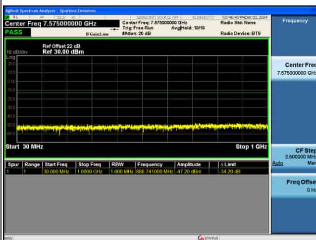
CSE_5G_n77(K)_30KHz_.PI2-BPSK_30M CH635666_1RB@1
