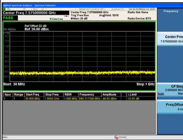
CSE_5G_n77(K)_30KHz_.PI2-BPSK_50M CH633334_1RB@1
