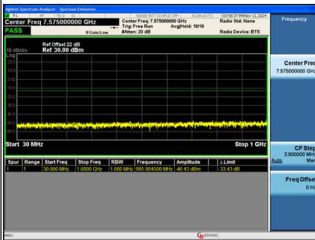
CSE_4G_B43_64QAM_15M CH45090 1RB@0
