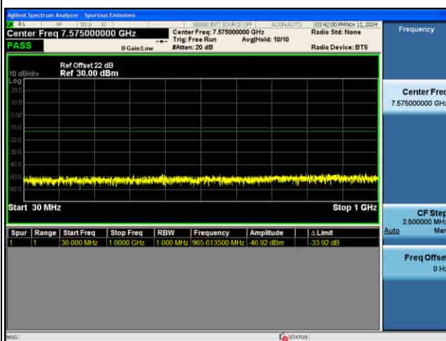
CSE_4G_B43_.QPSK_10M CH45540 1RB@0
