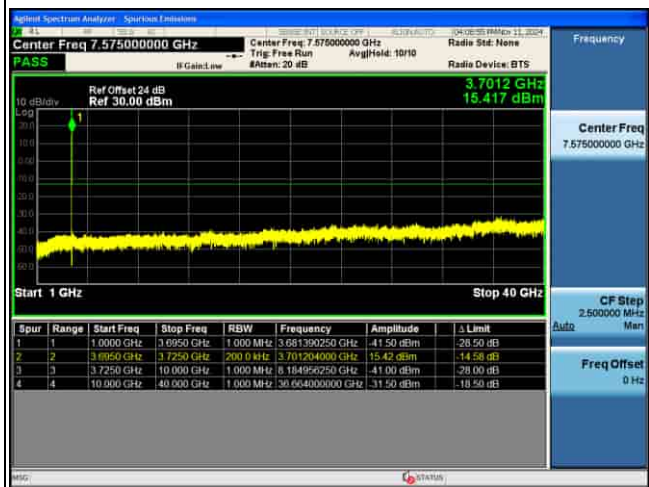
CSE_4G_B43_256QAM_20M CH45090 1RB@0_
