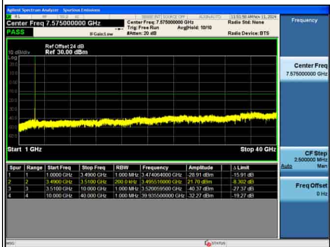
CSE_4G_B42_16QAM_10M CH43040 1RB@0_
