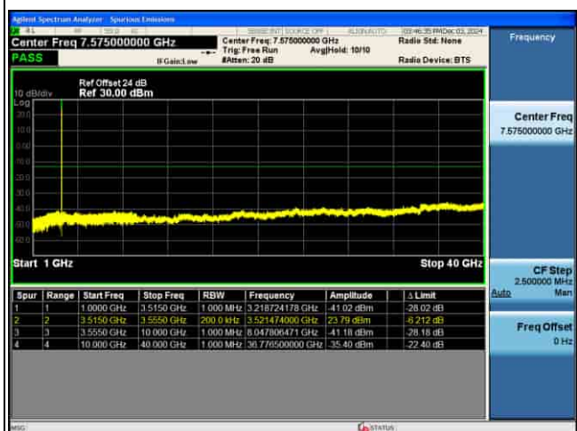
CSE_5G_n77(K)_30KHz_.PI2-BPSK_30M CH635666_1RB@1_
