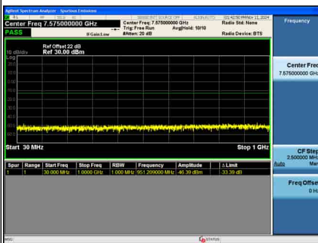
CSE_4G_B42_.QPSK_20M CH42990 1RB@0
