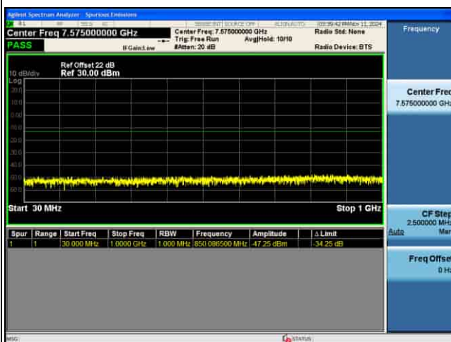
CSE_4G_B43_16QAM_10M CH45540 1RB@0
