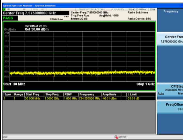
CSE_4G_B42_.QPSK_20M CH42590 1RB@0
