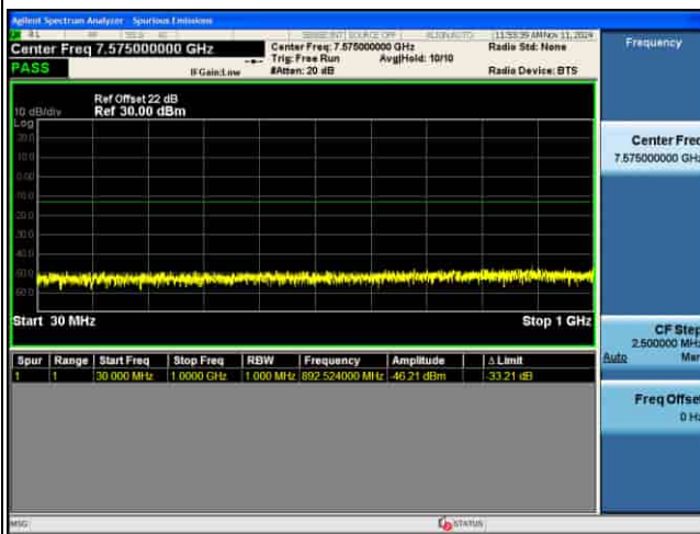
CSE_4G_B42_.QPSK_10M CH42590 1RB@0
