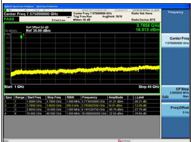
CSE_4G_B43_64QAM_15M CH45515 1RB@0_
