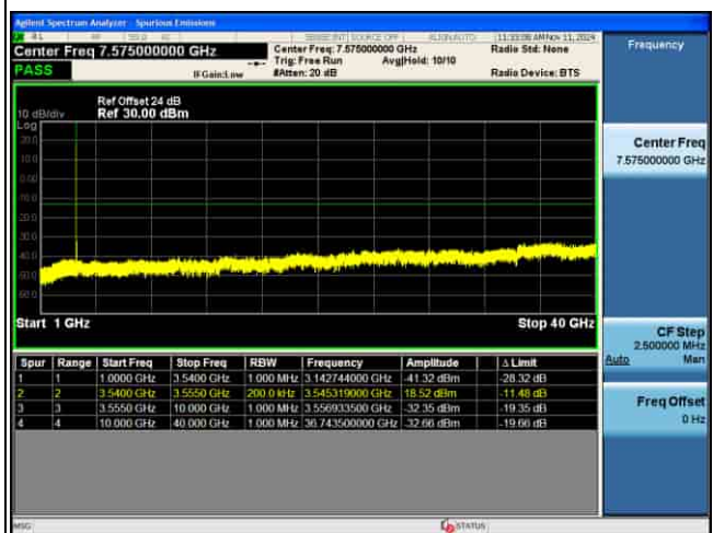
CSE_4G_B42_256QAM_5M CH43065 1RB@0_
