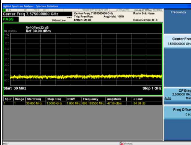
CSE_5G_n77(K)_30KHz_.PI2-BPSK_60M CH634666_1RB@1
