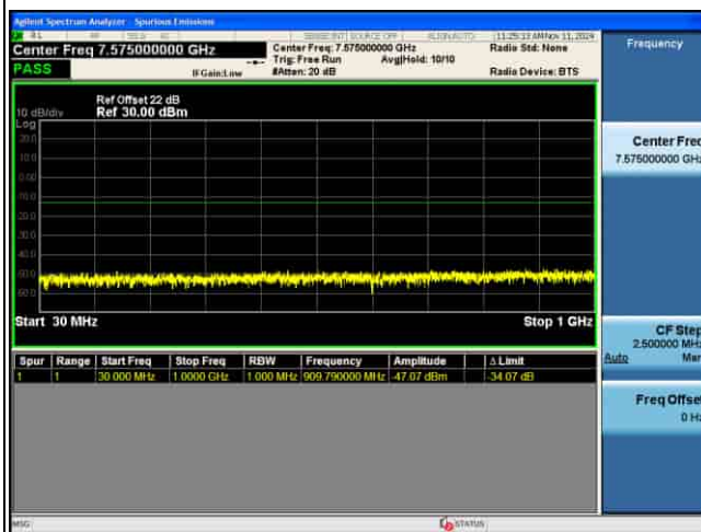
CSE_4G_B42_16QAM_5M CH43065 1RB@0
