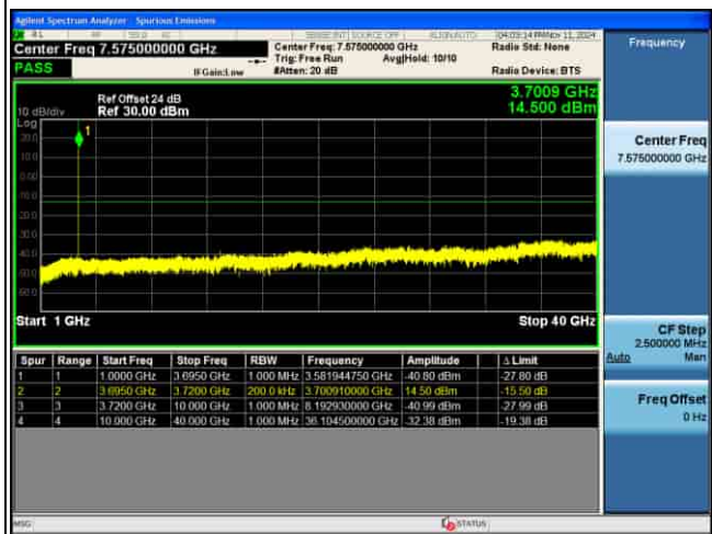
CSE_4G_B43_256QAM_15M CH45090 1RB@0_
