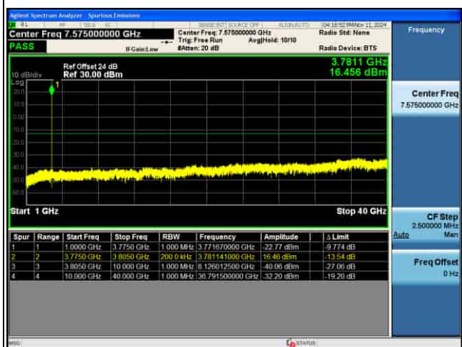
CSE_4G_B43_16QAM_20M CH45490 1RB@0_
