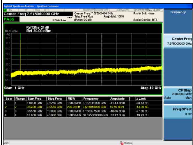
CSE_4G_B42_256QAM_20M CH42990 1RB@0_
