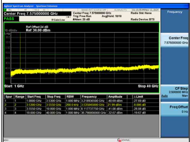
CSE_4G_B42_16QAM_15M CH43015 1RB@0_
