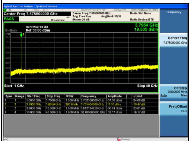
CSE_4G_B43_64QAM_5M CH45565 1RB@0_
