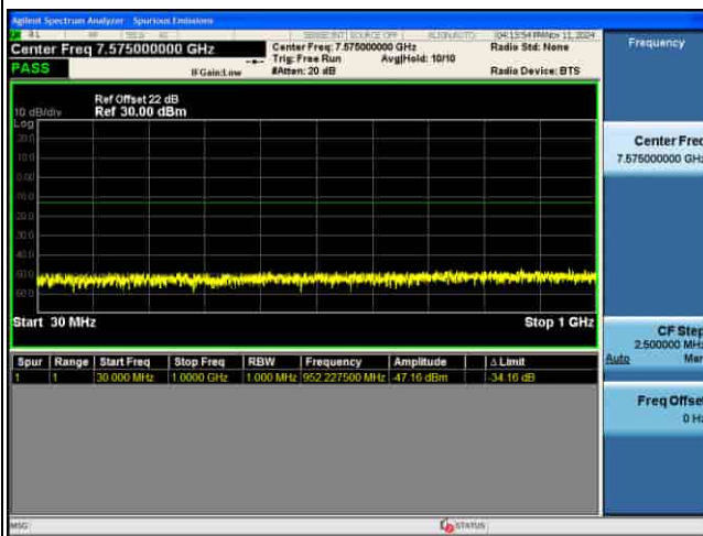
CSE_4G_B43_64QAM_20M CH45090 1RB@0
