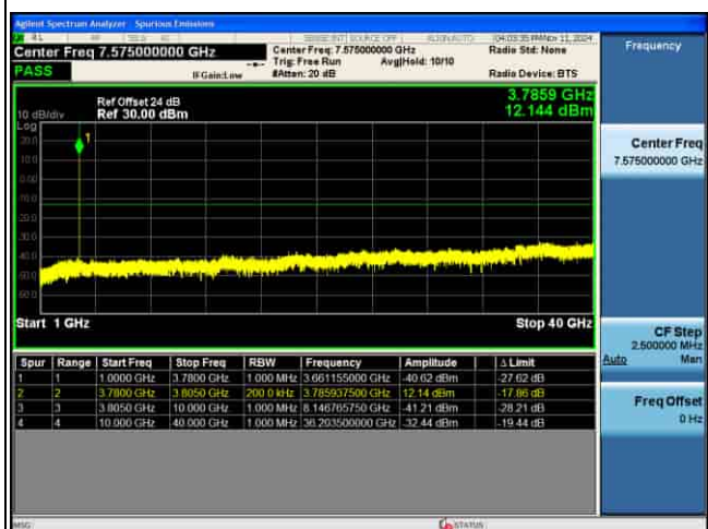
CSE_4G_B43_256QAM_15M CH45515 1RB@0_
