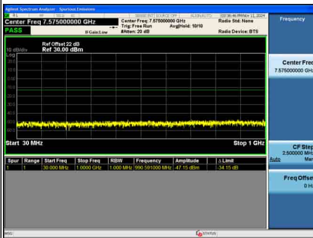
CSE_4G_B43_16QAM_10M CH45090 1RB@0
