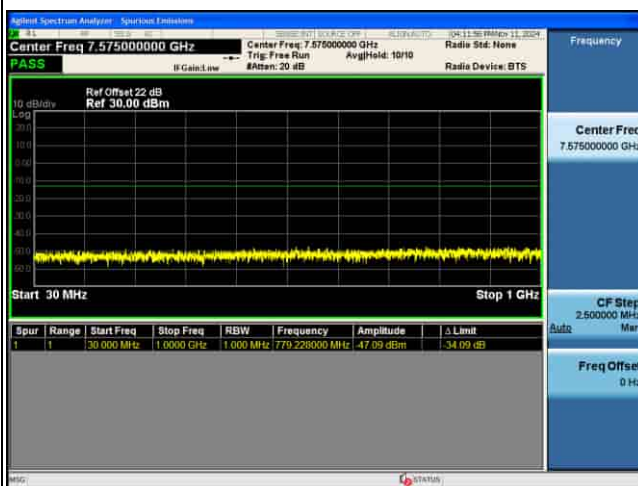
CSE_4G_B43_256QAM_20M CH45490 1RB@0
