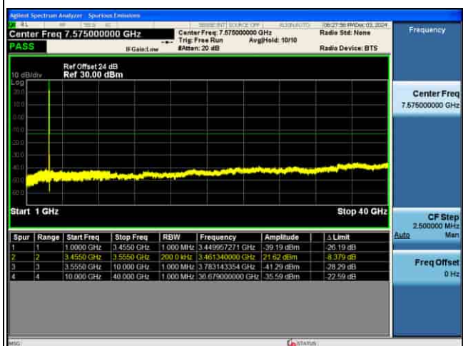
CSE_5G_n77(K)_30KHz_.PI2-BPSK_90M CH633666_1RB@1_
