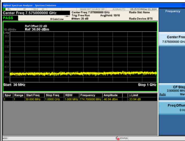
CSE_5G_n77(K)_30KHz_.PI2-BPSK_80M CH633334_1RB@1
