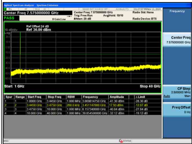
CSE_4G_B42_256QAM_20M CH42590 1RB@0_
