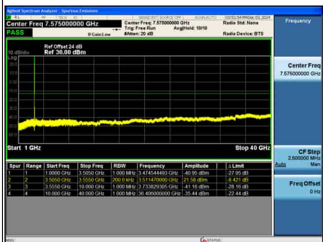
CSE_5G_n77(K)_30KHz_.PI2-BPSK_40M CH635332_1RB@1_
