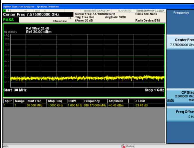
CSE_4G_B43_256QAM_5M CH45565 1RB@0
