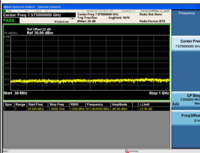
CSE_4G_B43_64QAM_10M CH45540 1RB@0
