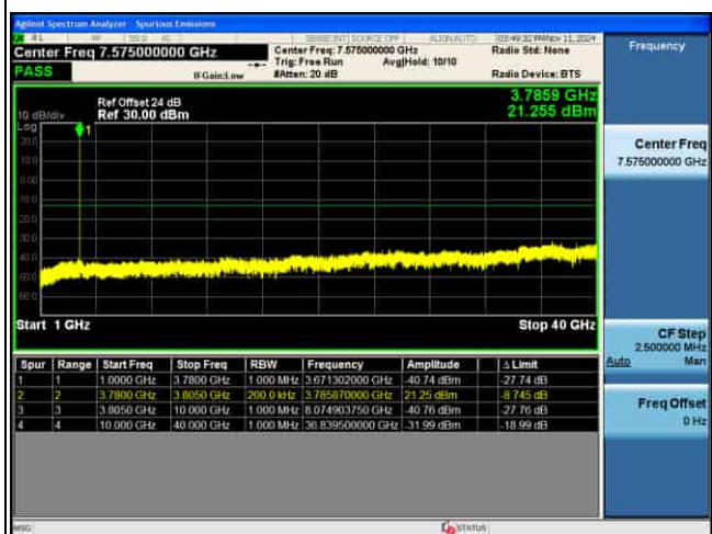
CSE_4G_B43_.QPSK_15M CH45515 1RB@0_
