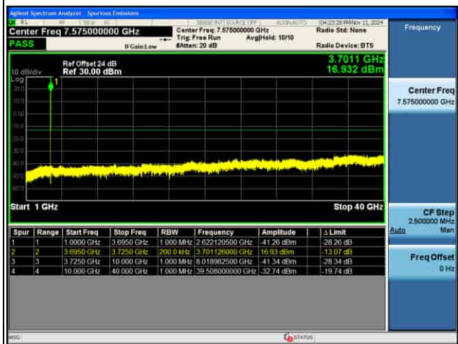
CSE_4G_B43_.QPSK_20M CH45090 1RB@0_
