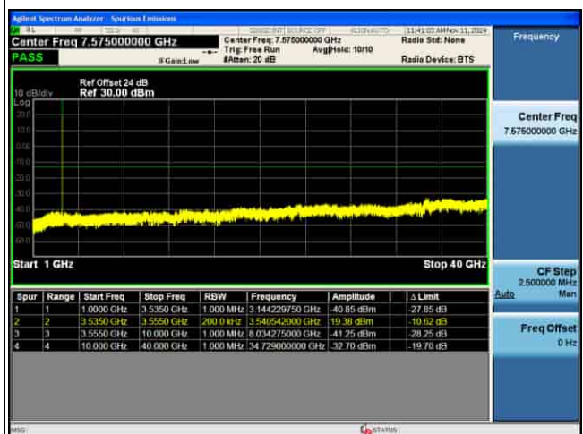
CSE_4G_B42_256QAM_10M CH43040 1RB@0_
