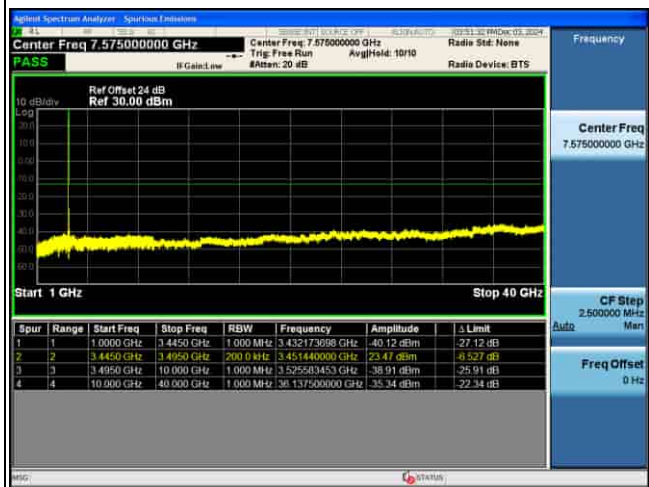
CSE_5G_n77(K)_30KHz_.PI2-BPSK_40M CH633334_1RB@1_
