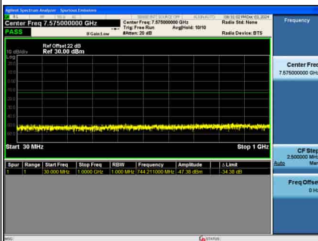
CSE_5G_n77(K)_30KHz_.PI2-BPSK_90M CH633666_1RB@1
