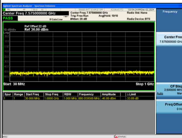
CSE_5G_n77(K)_30KHz_.PI2-BPSK_40M CH635332_1RB@1
