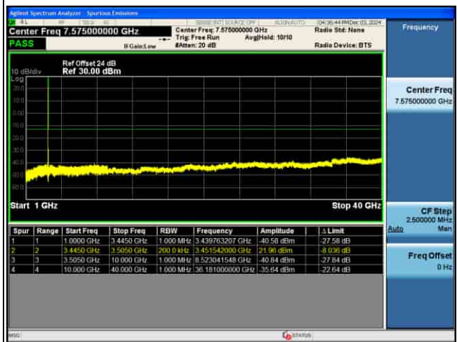
CSE_5G_n77(K)_30KHz_.PI2-BPSK_50M CH633334_1RB@1_
