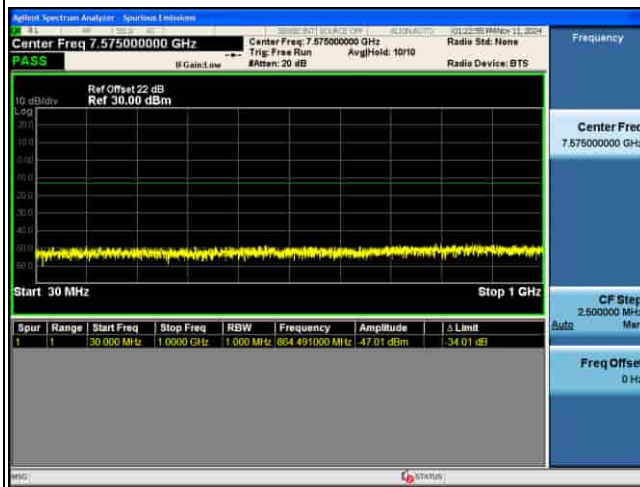
CSE_4G_B42_256QAM_15M CH42590 1RB@0
