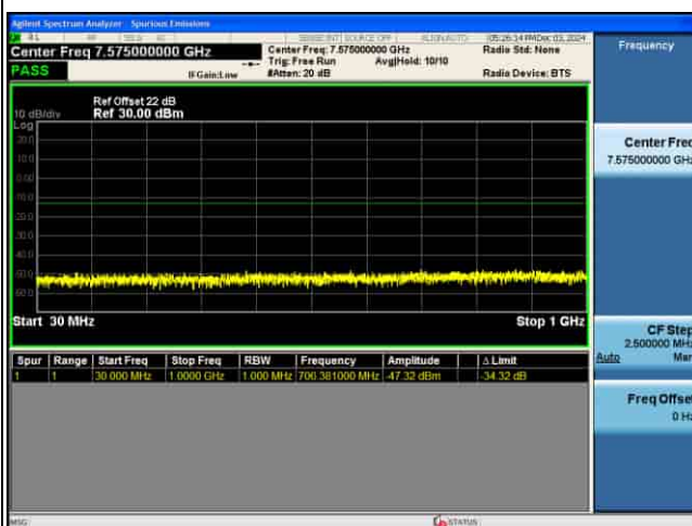
CSE_5G_n77(K)_30KHz_.PI2-BPSK_80M CH634000_1RB@1
