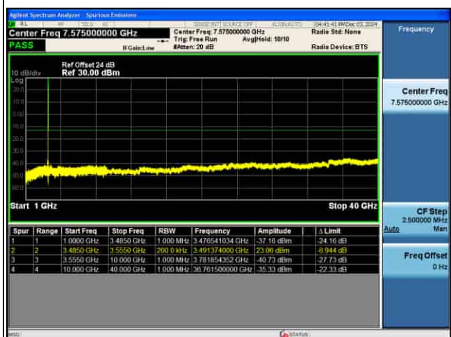
CSE_5G_n77(K)_30KHz_.PI2-BPSK_60M CH634666_1RB@1_
