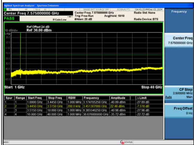
CSE_5G_n77(K)_30KHz_.PI2-BPSK_60M CH633334_1RB@1_
