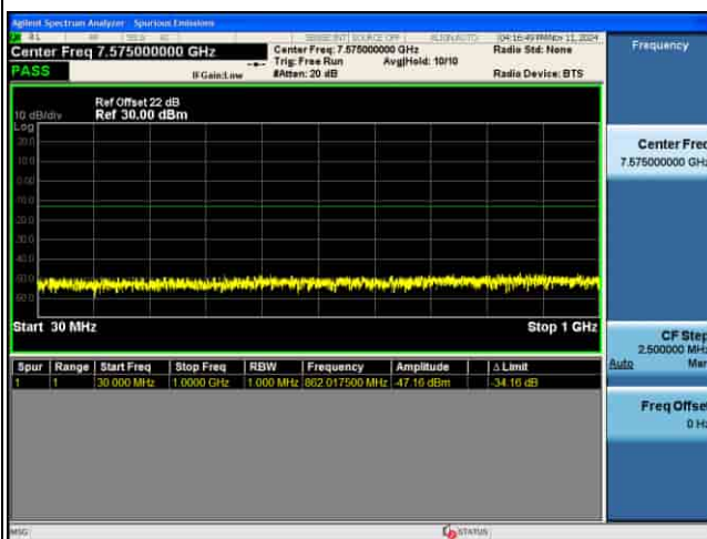
CSE_4G_B43_64QAM_20M CH45490 1RB@0
