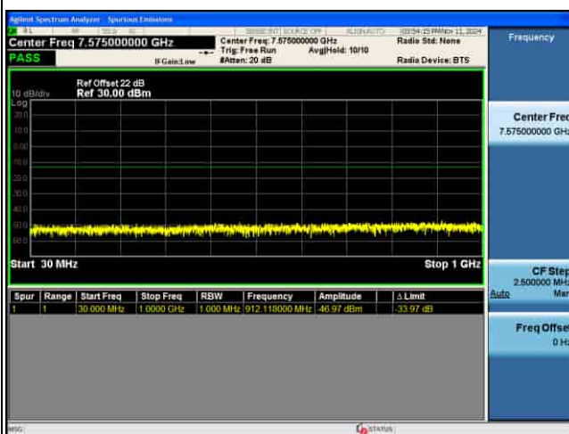
CSE_4G_B43_16QAM_15M CH45515 1RB@0
