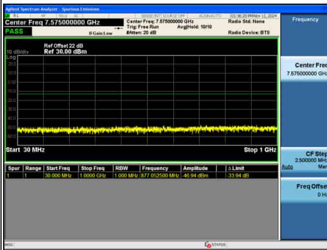
CSE_4G_B42_16QAM_20M CH42590 1RB@0
