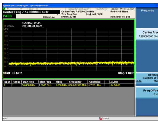
CSE_4G_B42_64QAM_5M CH42590 1RB@0
