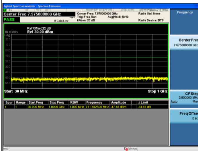
CSE_4G_B42_256QAM_15M CH43015 1RB@0
