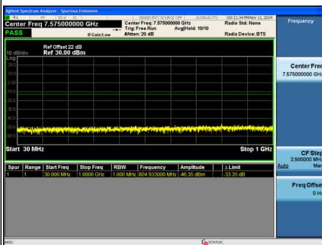
CSE_4G_B43_256QAM_10M CH45540 1RB@0
