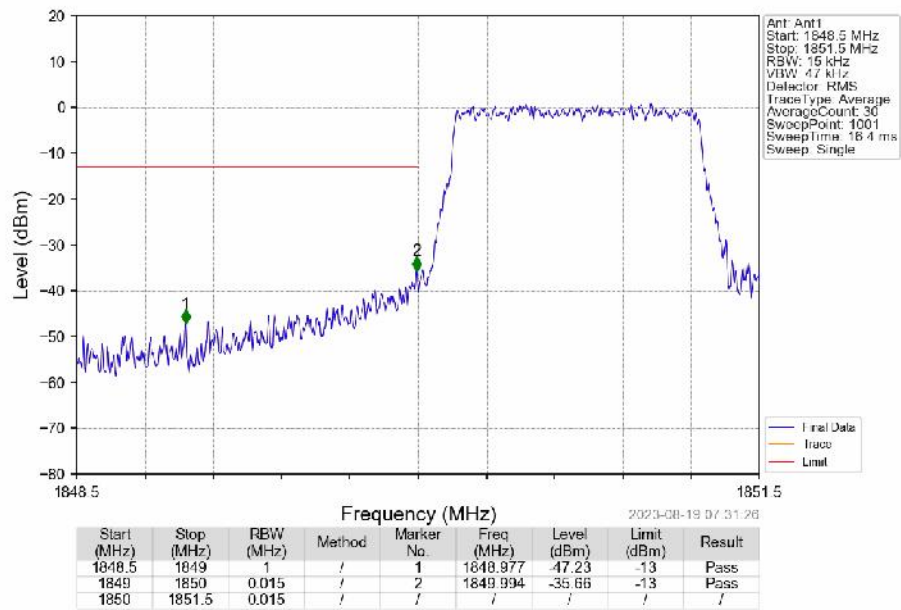
Band2_1.4MHz_QPSK_LCH_1850.7MHz_RB_6_0_NTNV
