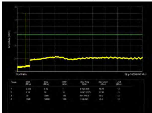
LTE Band 71 5MHz CH-High 9kHz~10GHz
