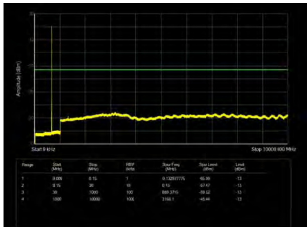
LTE Band 71 5MHz CH- Middle 9kHz~10GHz
