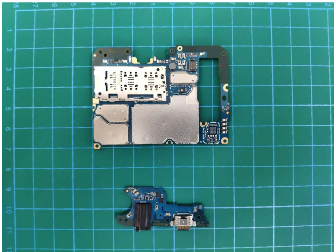
PCB06
