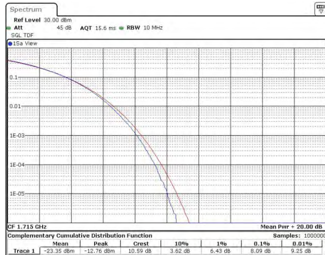
Band66-10MHz-16QAM-132022-50RB#0
