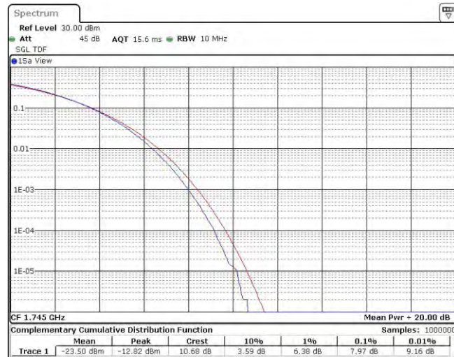
Band66-15MHz-QPSK-132597-1RB#0
