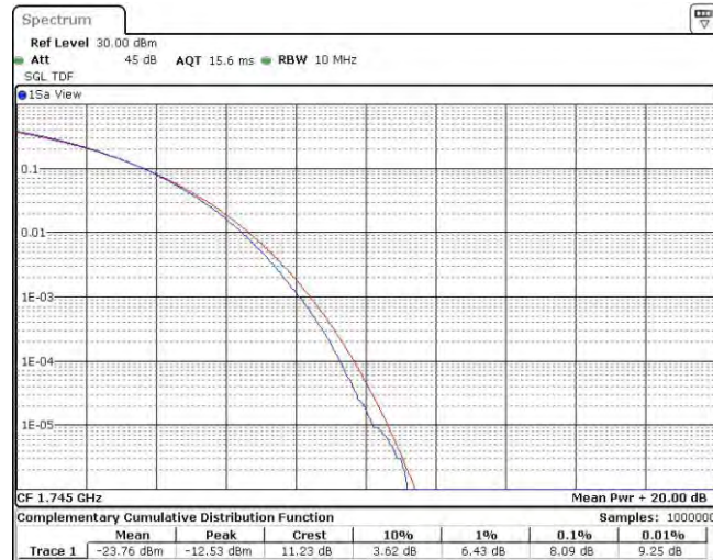
Band66-10MHz-QPSK-132322-50RB#0
