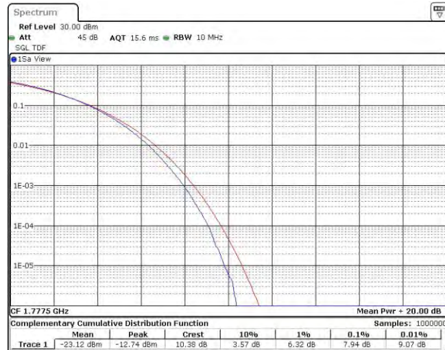
Band66-10MHz-QPSK-132022-1RB#0
