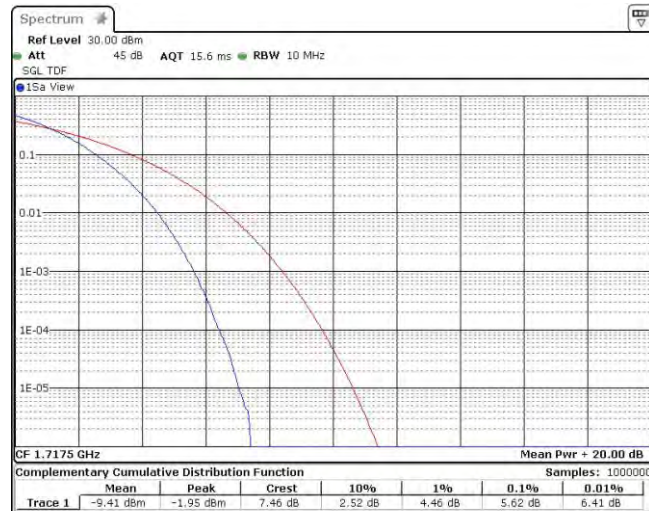
Band66-15MHz-QPSK-132047-75RB#0
