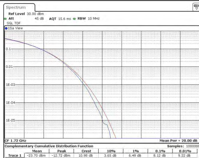
Band66-20MHz-16QAM-132322-1RB#0
