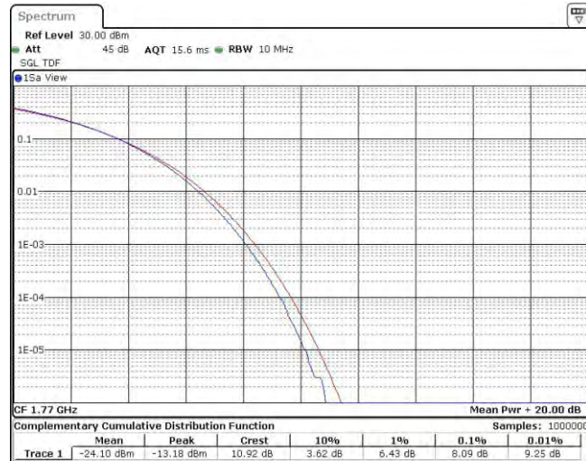
Band66-20MHz-16QAM-132072-1RB#0
