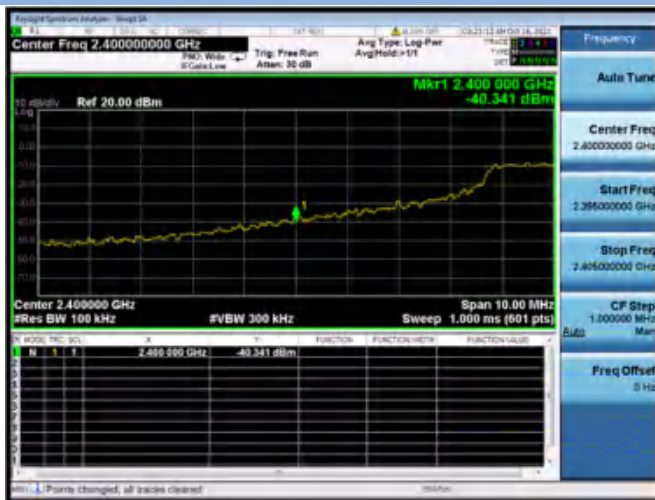
802.11VHT-40 MHz CHANNEL 3, Carrier level
