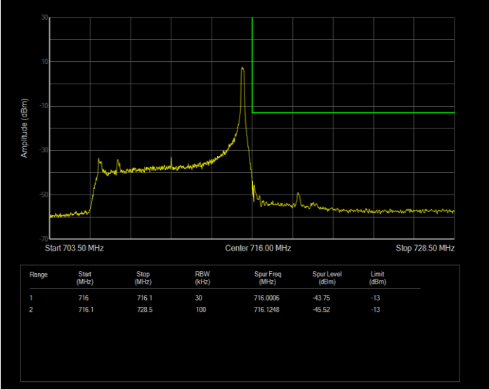
Band12 16QAM BW=10MHz Channel=23130 RB Size=27 Position=#0 Normal
