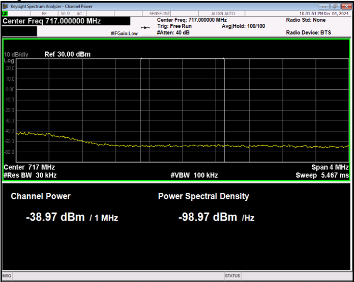
Band12 16QAM BW=10MHz Channel=23130 RB Size=27 Position=#0 Extended
