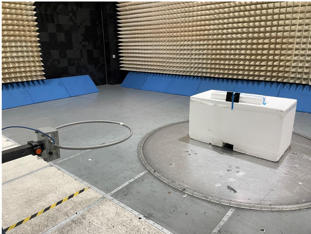
RSE (150kHz – 30MHz)
