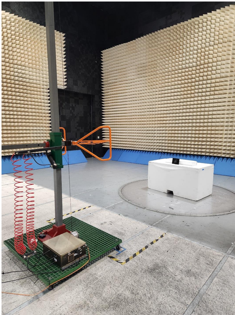
Unintentional Emissions and RSE (30MHz – 1GHz)
