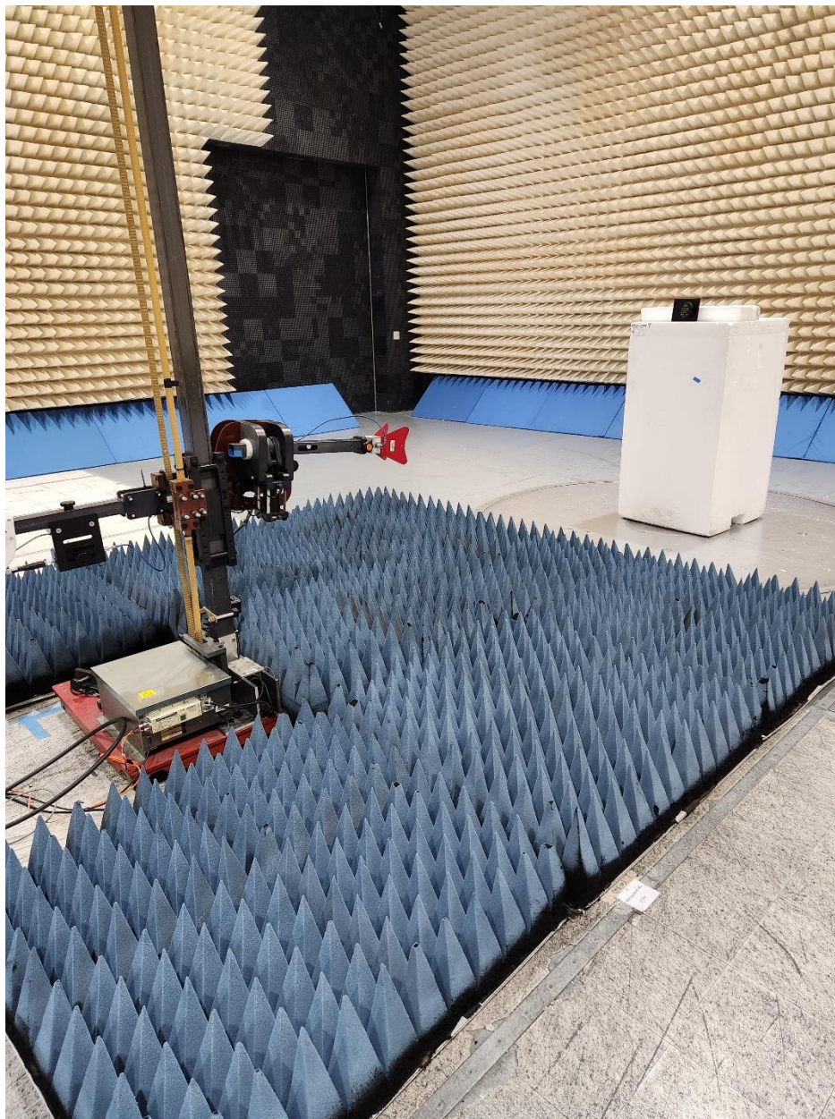
RSE (1GHz – 18GHz)
