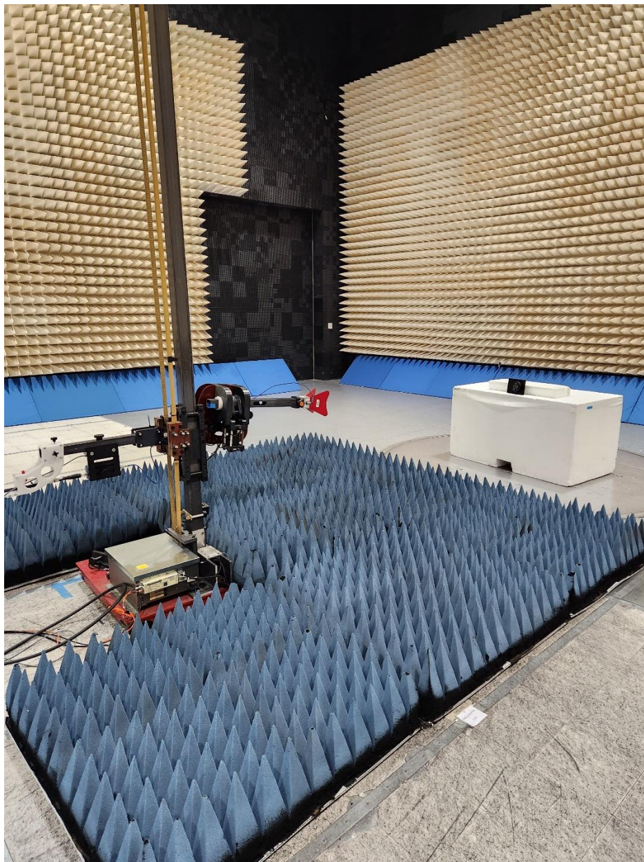
Unintentional Emissions (1GHz – 18GHz)
